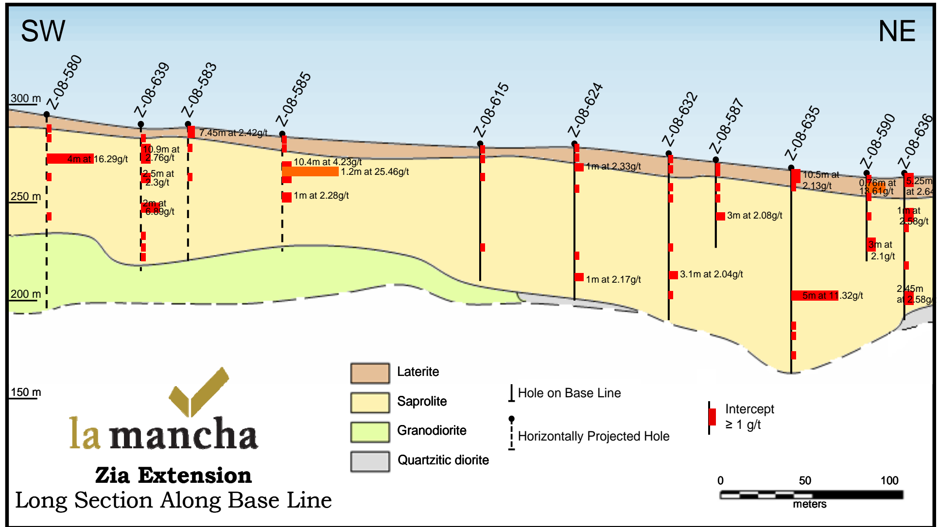
Figure 3 Cross section along base line
