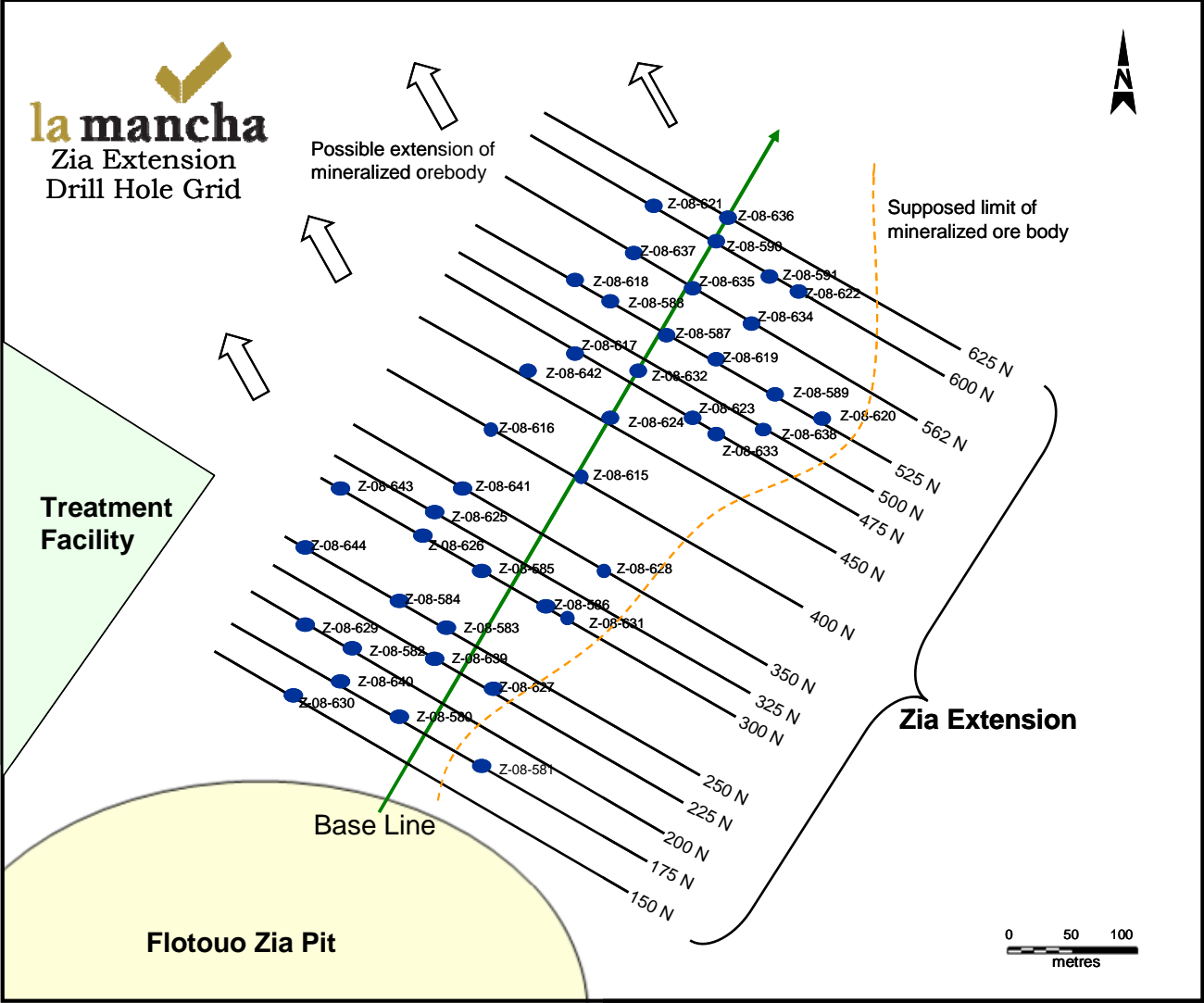
Figure 2 Zia extension anomaly: location of drill holes on 50-m gridlines
