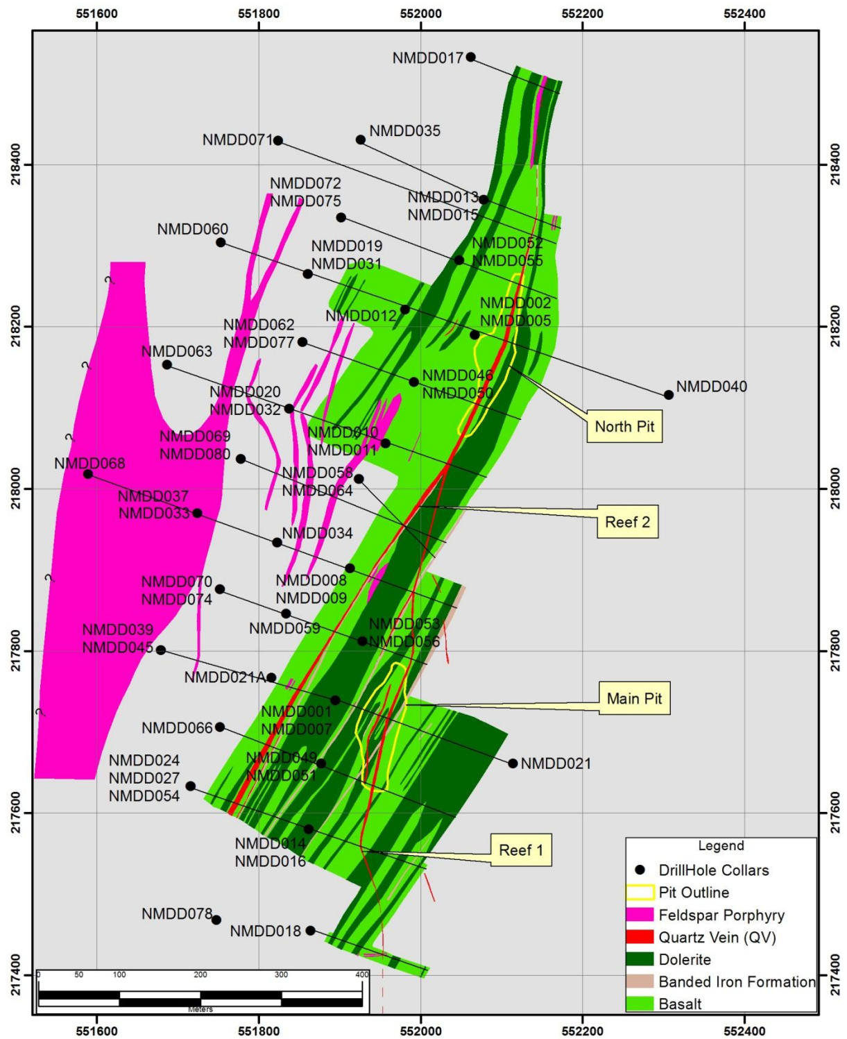
Figure 1 – Geology of the Main and North Pit areas, Makapela
