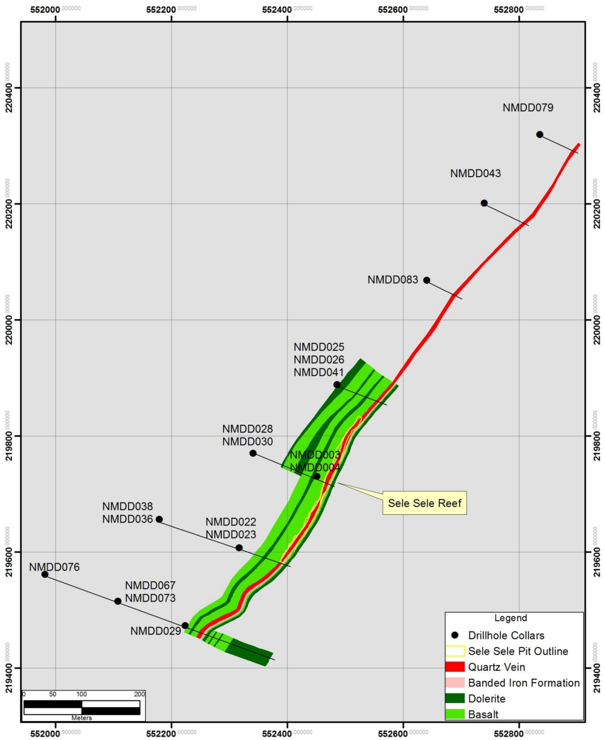
Figure 2 – Geology of the Sele Sele area, Makapela
