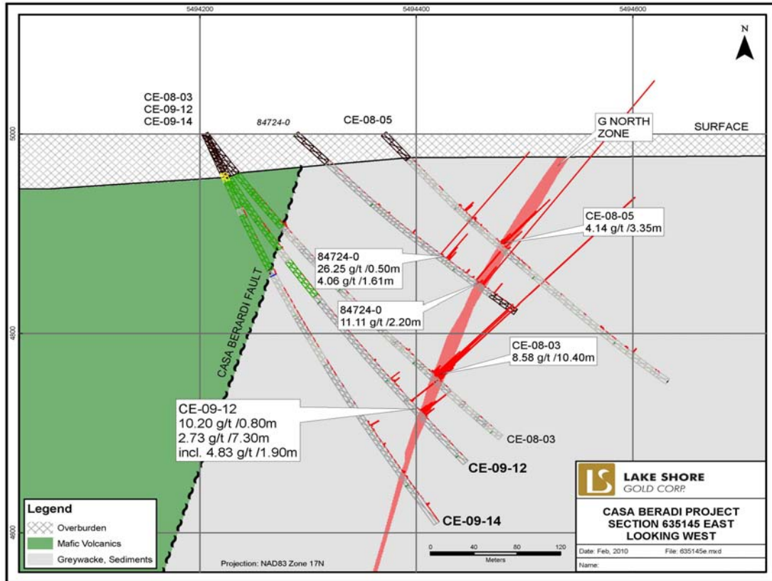
Figure 3. Cross Section
