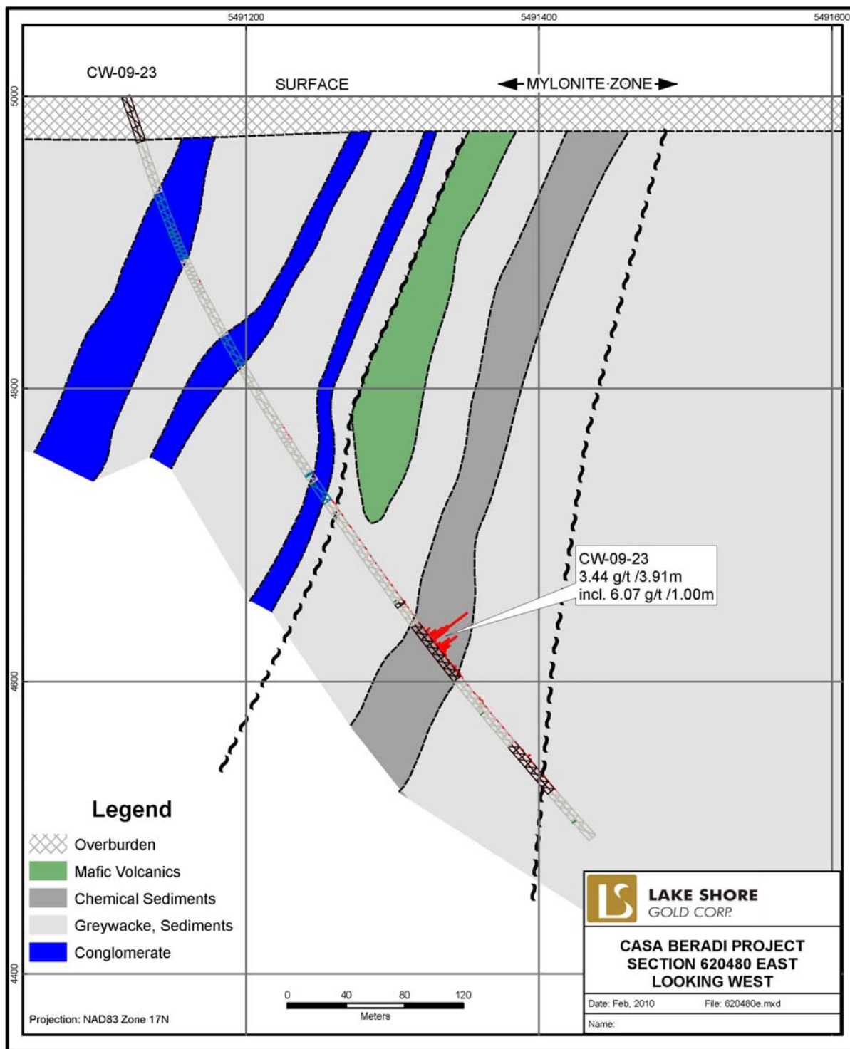
Figure 4. Cross Section (2)
