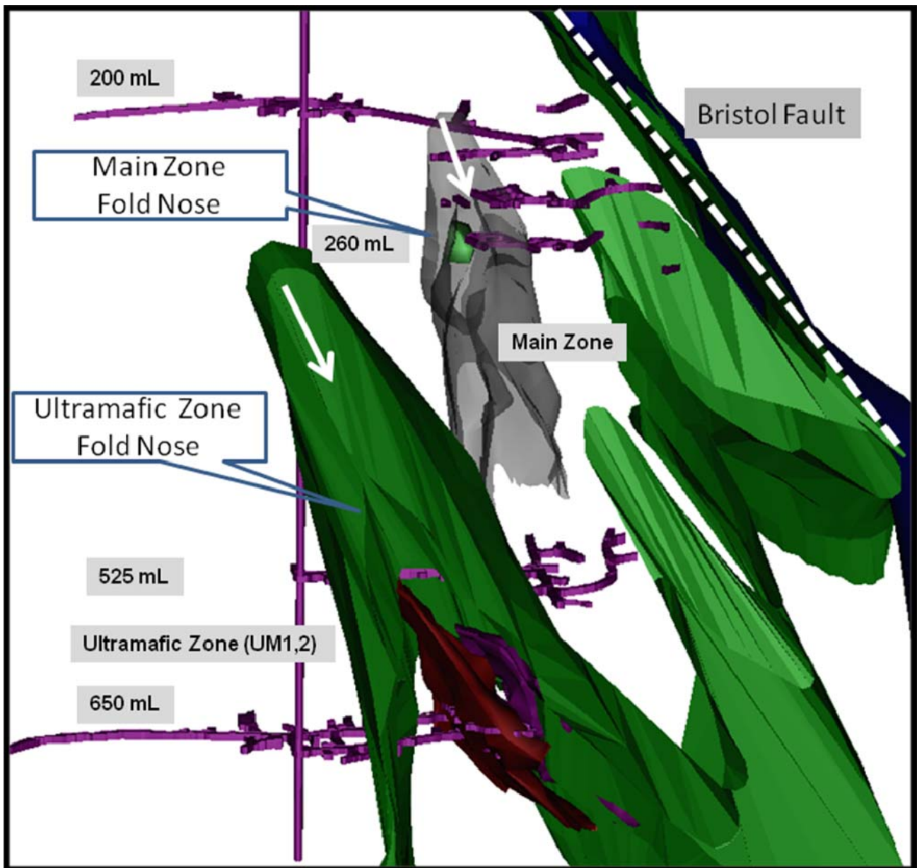
Figure 1. Isometric View
