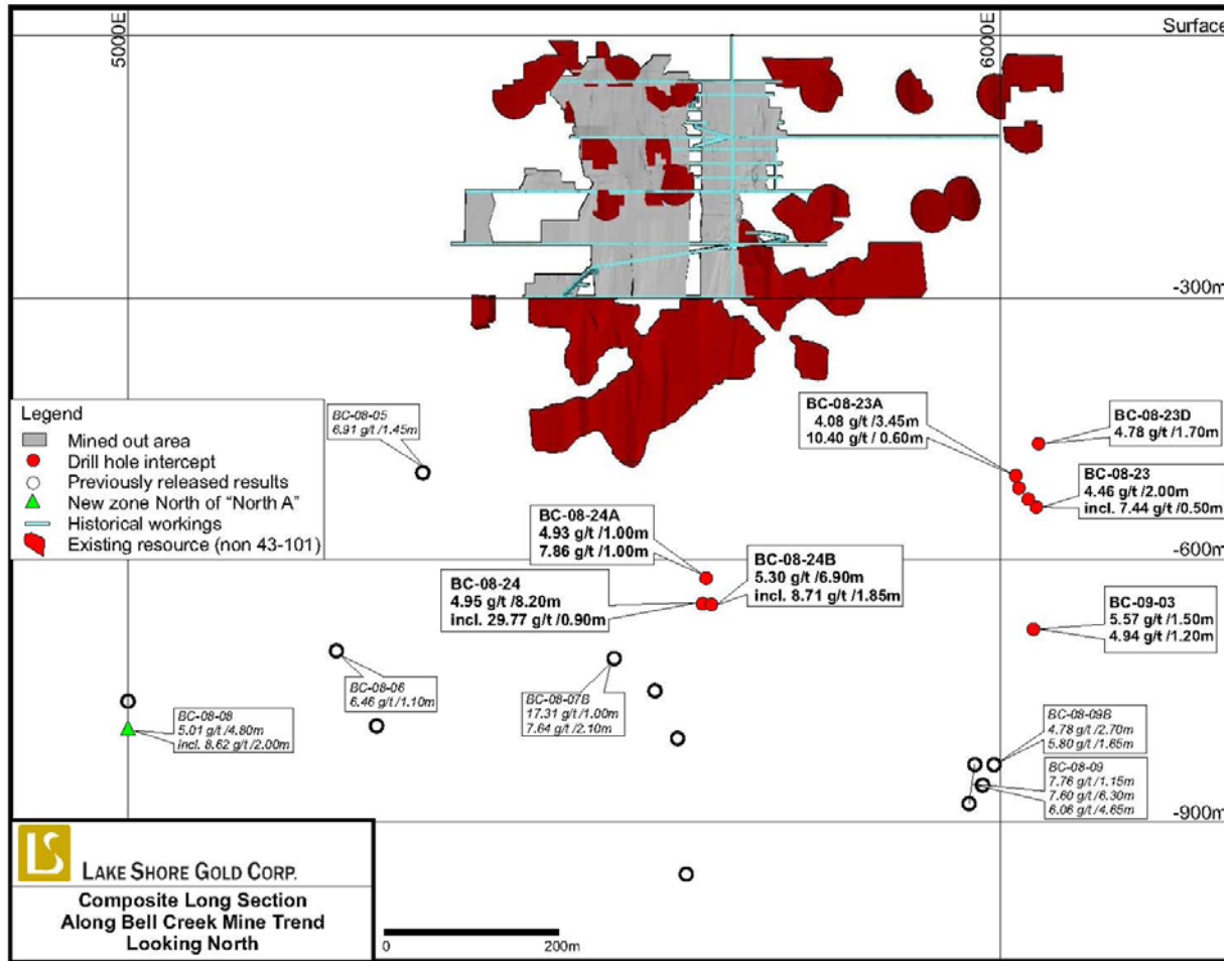
Figure 4. Long Section (Bell Creek)
