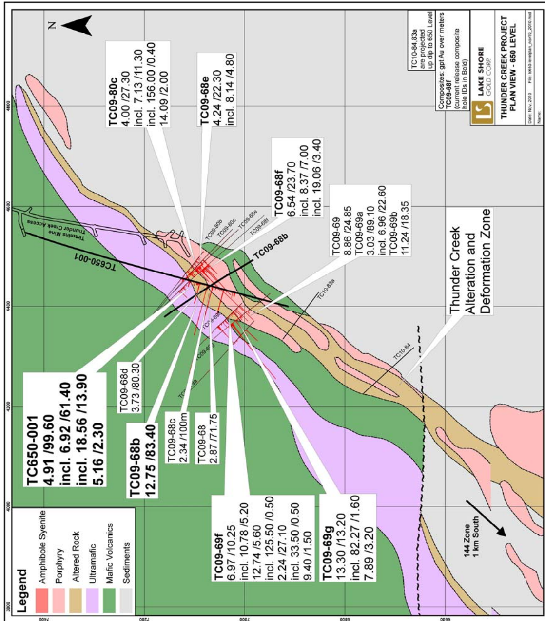
Figure 3. Plan View
