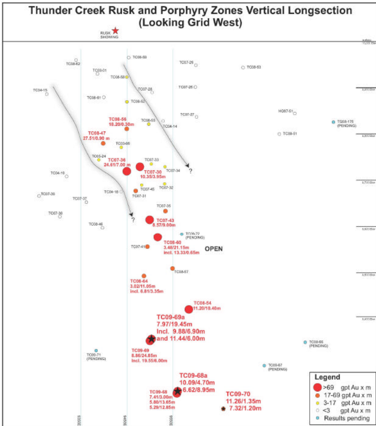
Figure 2. Long Section
