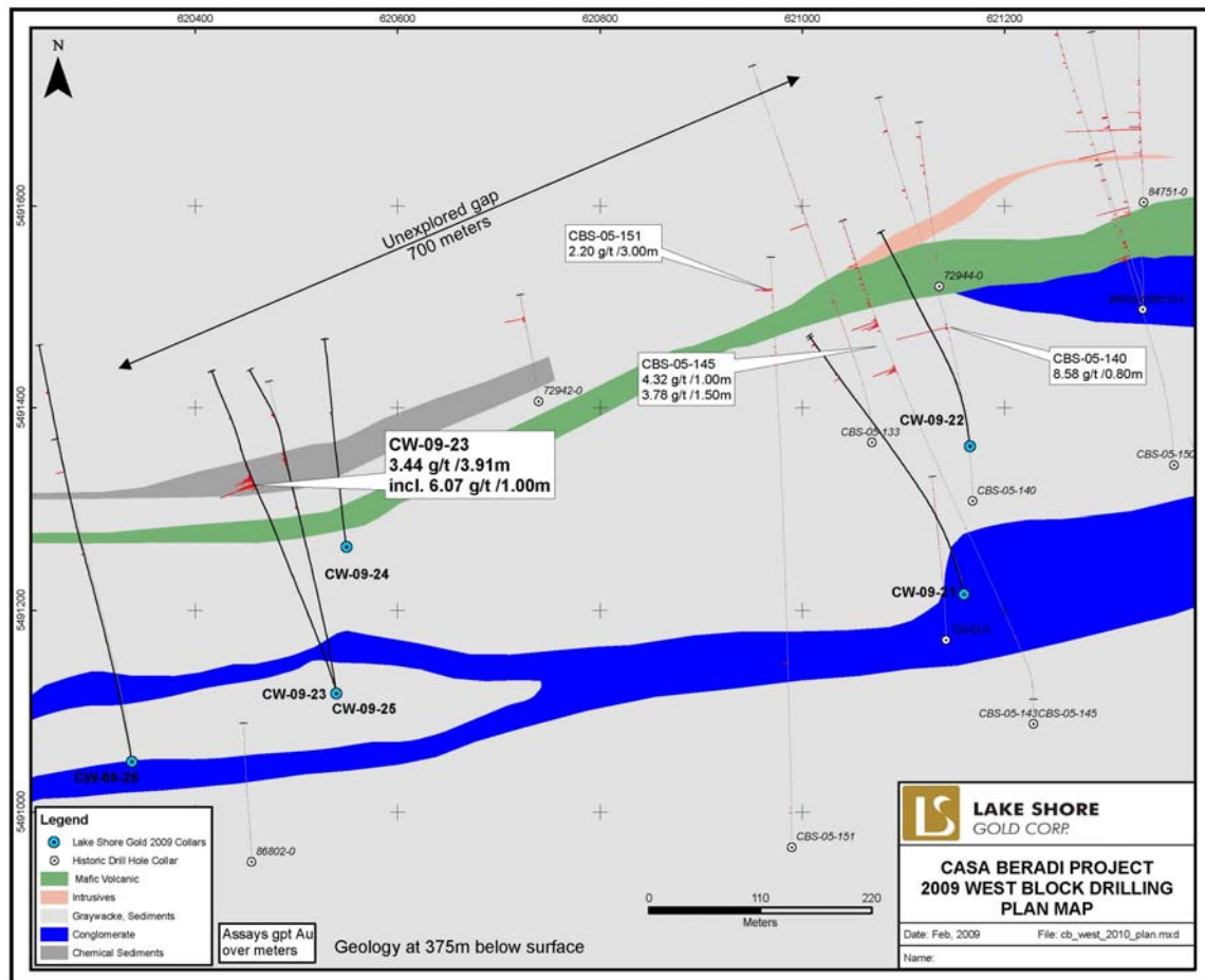
Figure 2. Plan View
