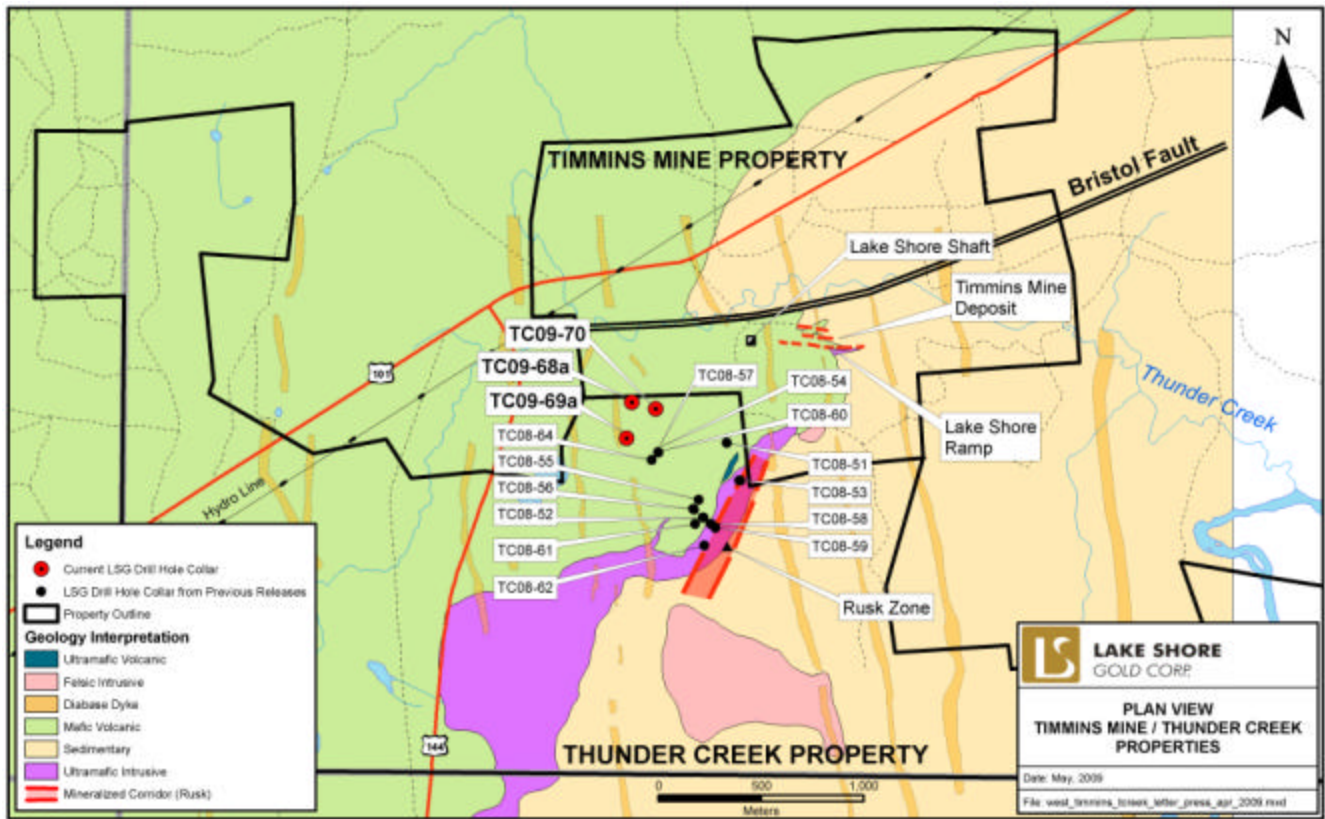
Figure 3. Plan View
