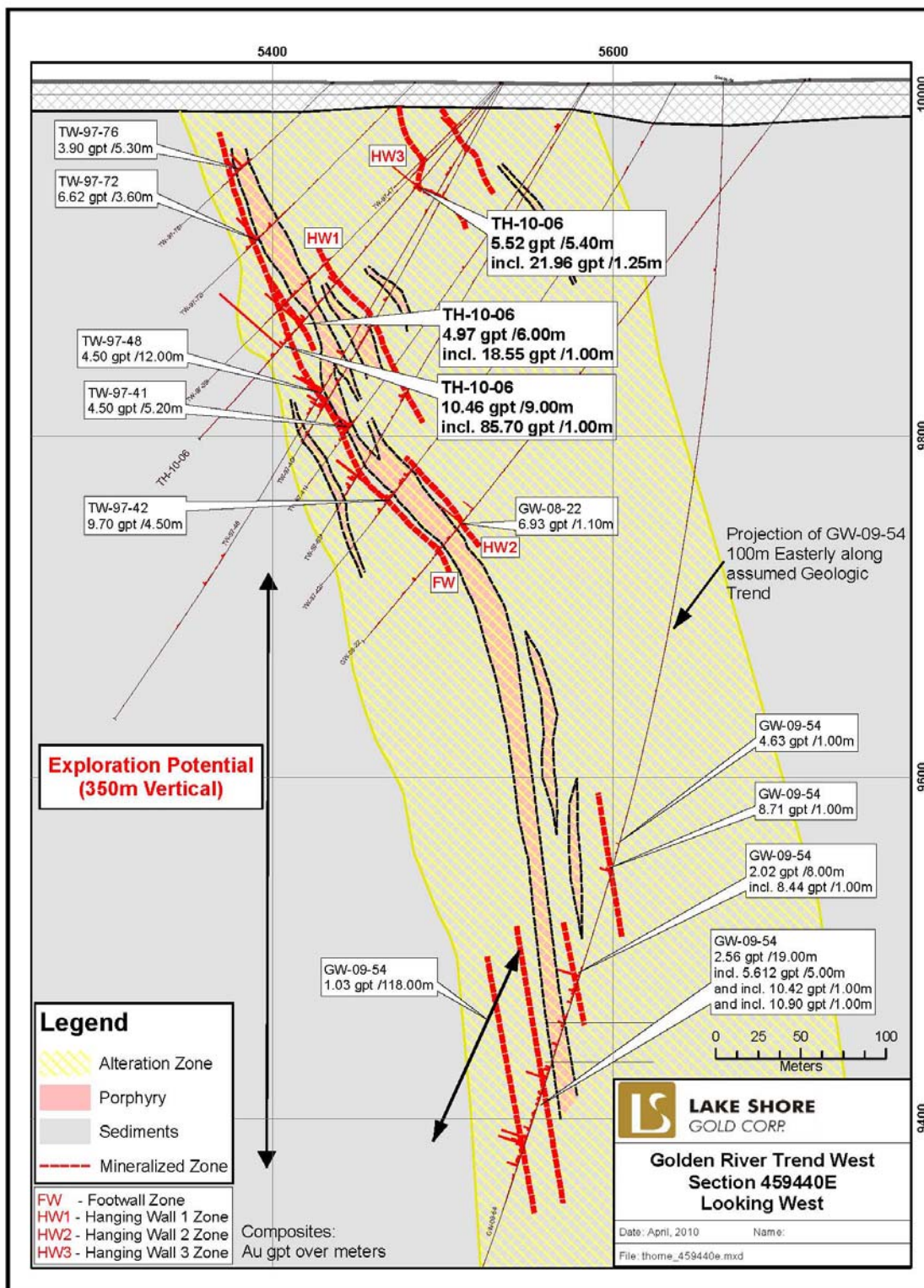
Figure 5. Cross Section – Gold River West
