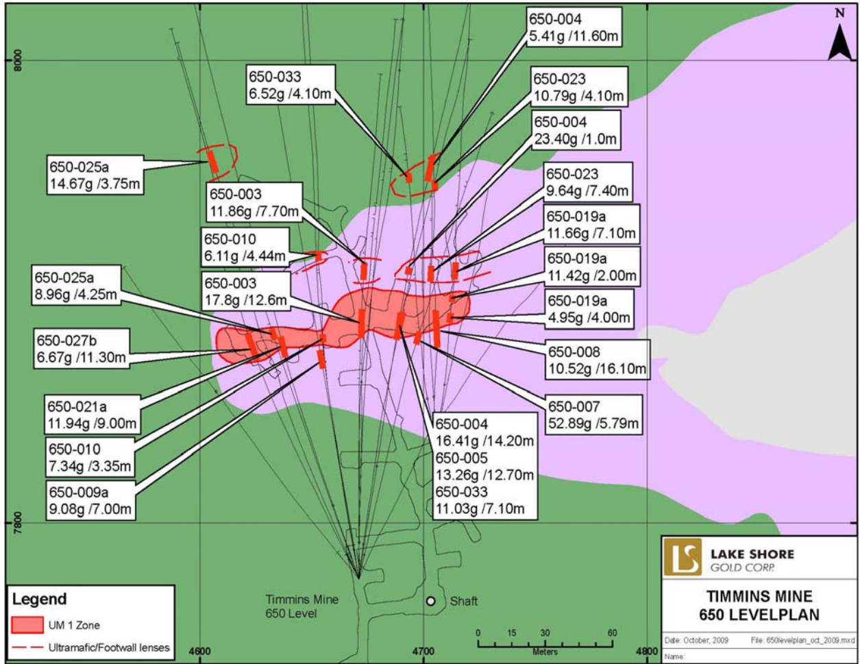
Figure 3. Plan View (Previously Reported Drilling)
