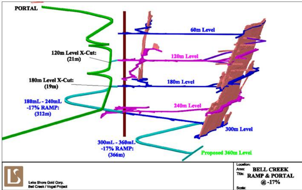
Figure 2. Bell Creek Ramp Portal (Conceptual View)
