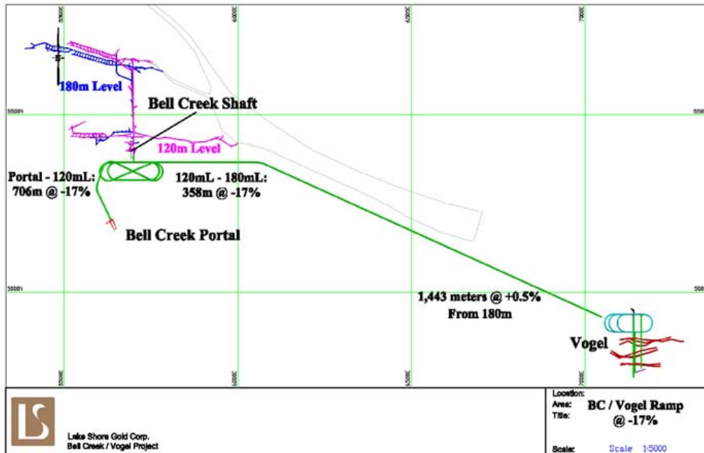
Figure 3. Ramp to Vogel (Conceptual View)
