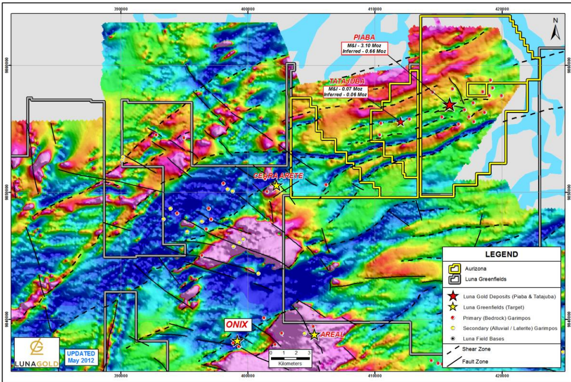
Figure 2. Location of the Onix target within the OXSZ. Overlain on total field magnetic grid.
