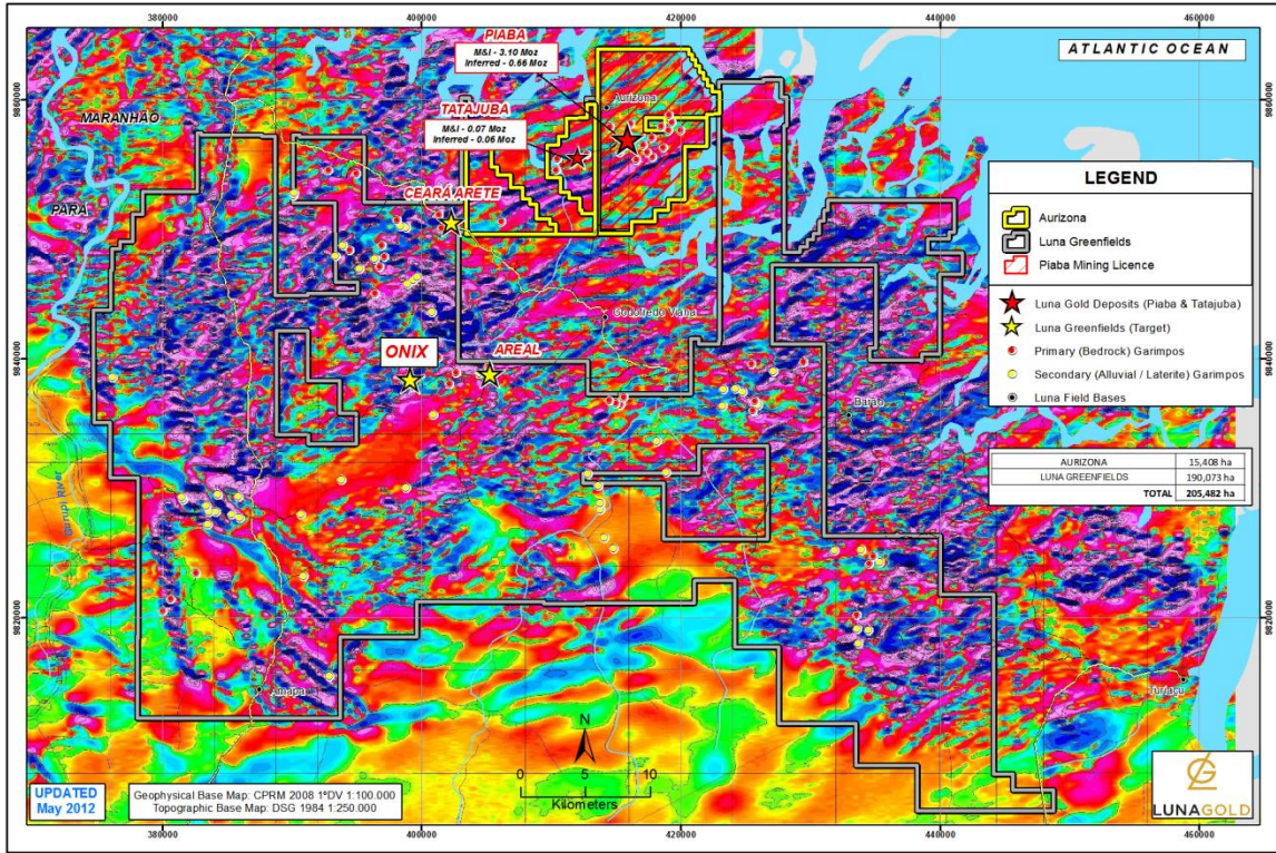
Figure 1. Location of the Onix target, Luna Greenfields project overlain on 1VD magnetic grid (CPRM, 2008).
