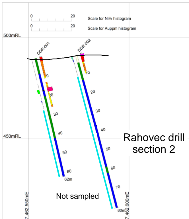
Figure 1 Drill hole cross-sections for Rahovec project Kosovo. See Figure 2 for locations. Gold grades on left hand side of drill trace and nickel grades on right hand side. Blue line indicates where drill hole was not sampled (most holes testing gold and copper zone, these hole sections to be dispatched for nickel analysis)
