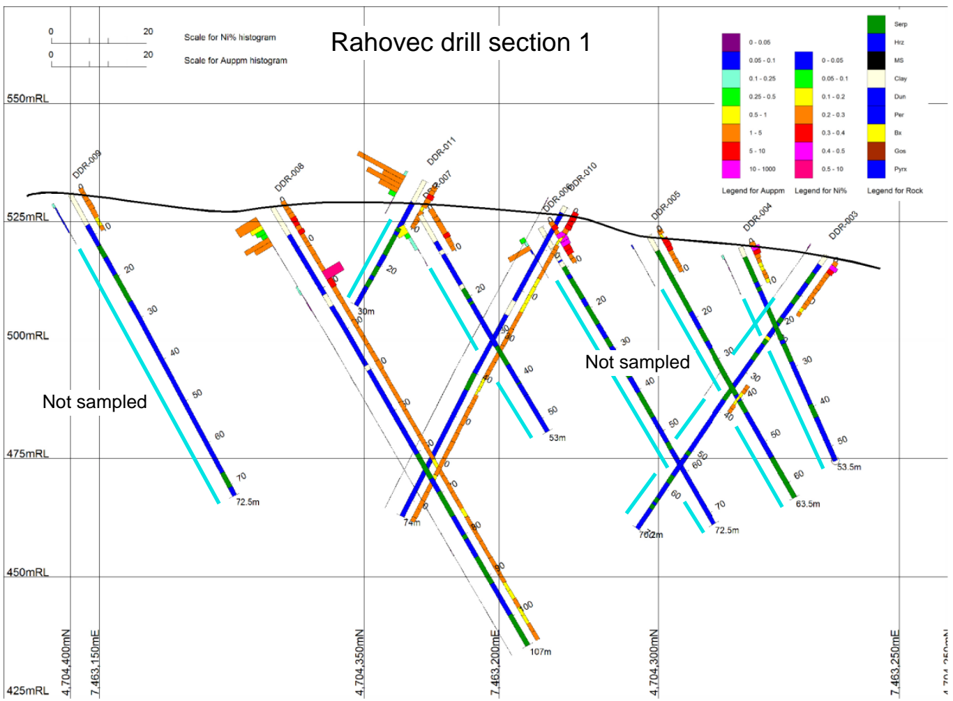
Figure 1 Drill hole cross-sections for Rahovec project Kosovo. See Figure 2 for locations. Gold grades on left hand side of drill trace and nickel grades on right hand side. Blue line indicates where drill hole was not sampled (most holes testing gold and copper zone, these hole sections to be dispatched for nickel analysis)
