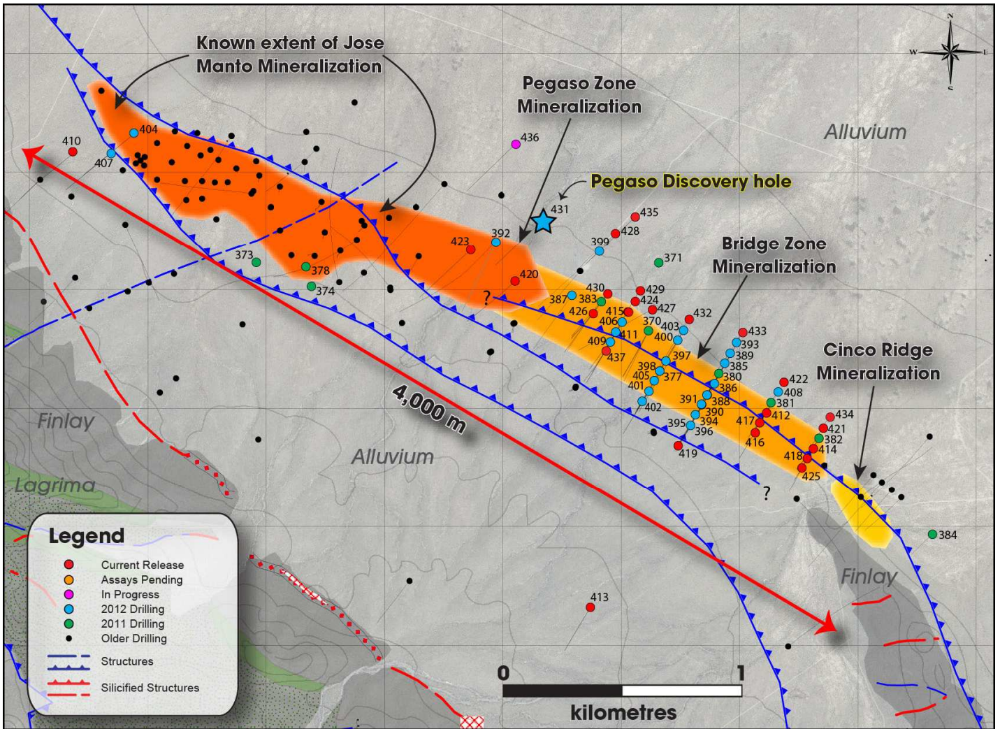
Figure 1: Plan map showing location of drillholes and surface projection of mineralization in the Bridge Zone and Jose Manto
