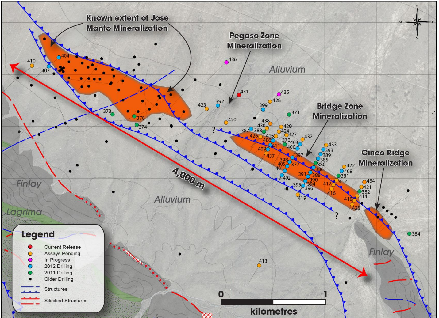
Diagram 3: Jose Manto – Cinco Ridge Mineralized Corridor (Bridge Zone)
