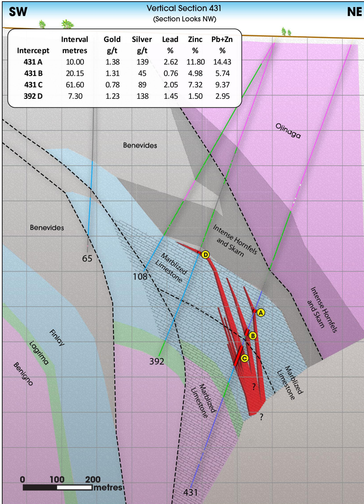
Diagram 1: Cross Section through Hole 431 with interpreted geology and massive sulphide body
