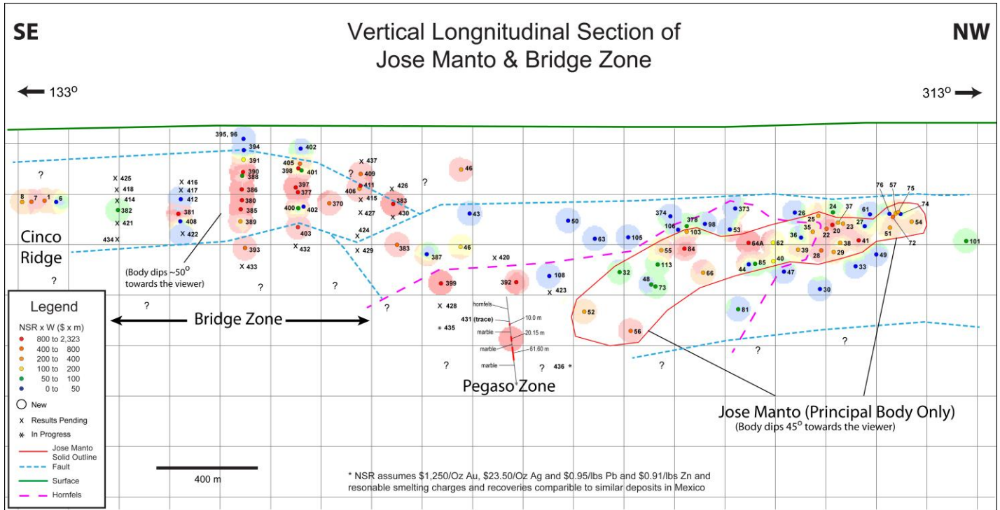
Diagram 2: Vertical Longitudinal Section showing Jose Manto and Bridge Zone areas
