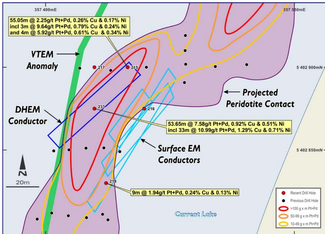
Figure 2. Recent drilling to test EM anomalies in the southern part of Current Lake (see Figure 3 for location of drilling in a regional context).
