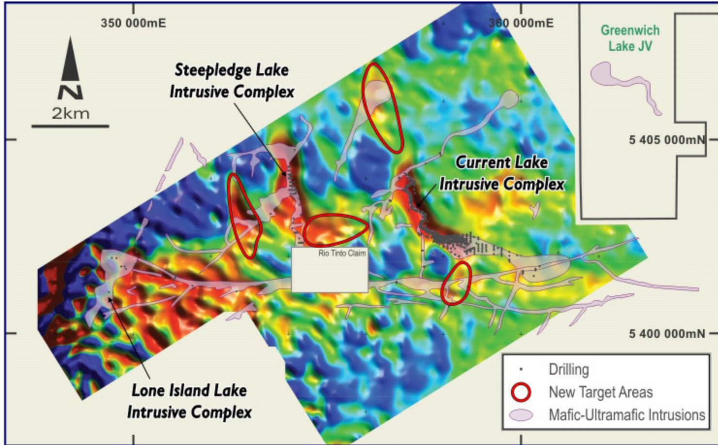
Figure 3. ZTEM survey of intrusive complexes in the TBN project showing new target areas.
