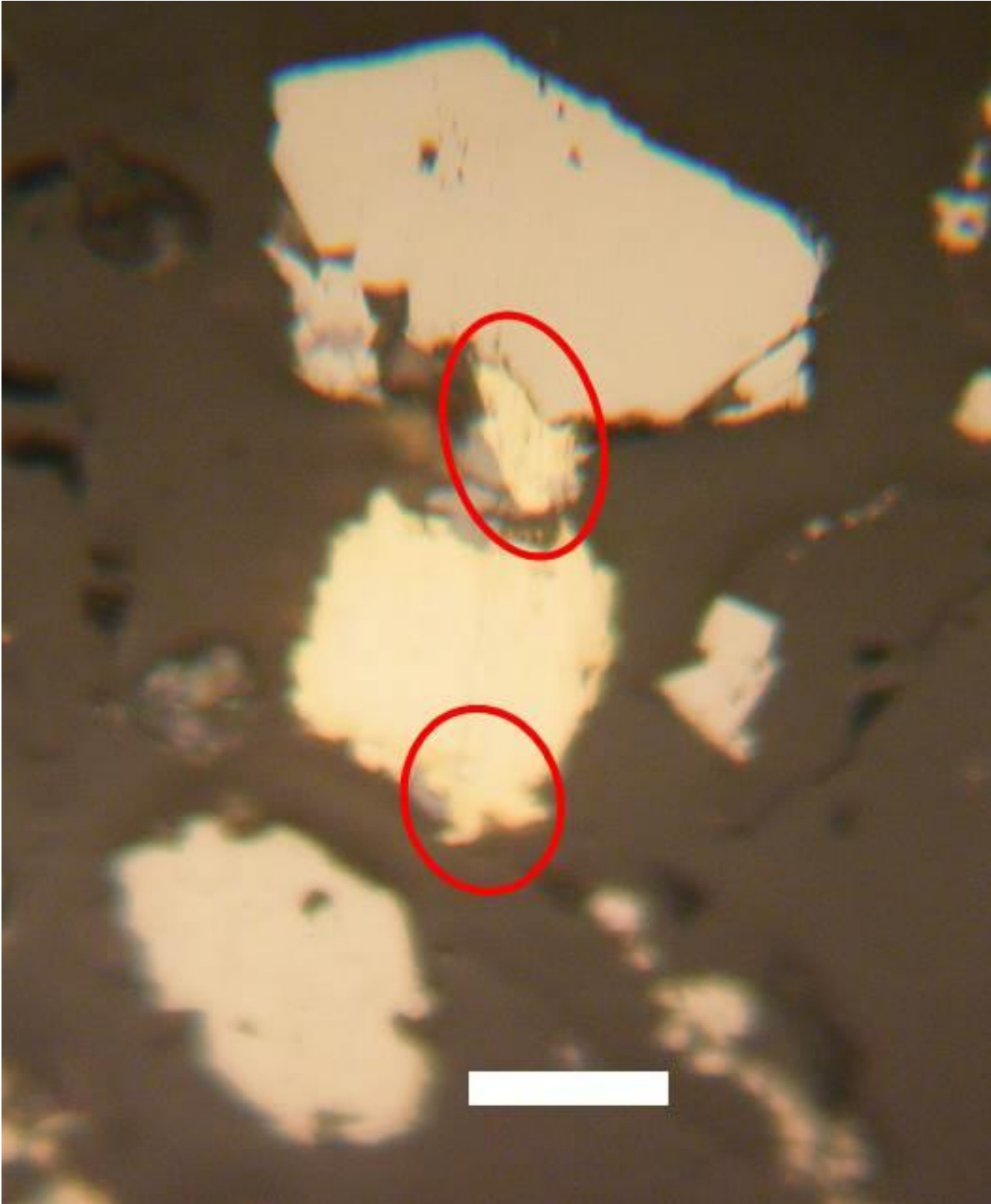
Image 1 - Occurrence of Free Gold Along Pyrite Grain Fracture and on Pyrite Grain Surface (gold grains are inside red circles, white scale bar equals 0.05 millimetres)
