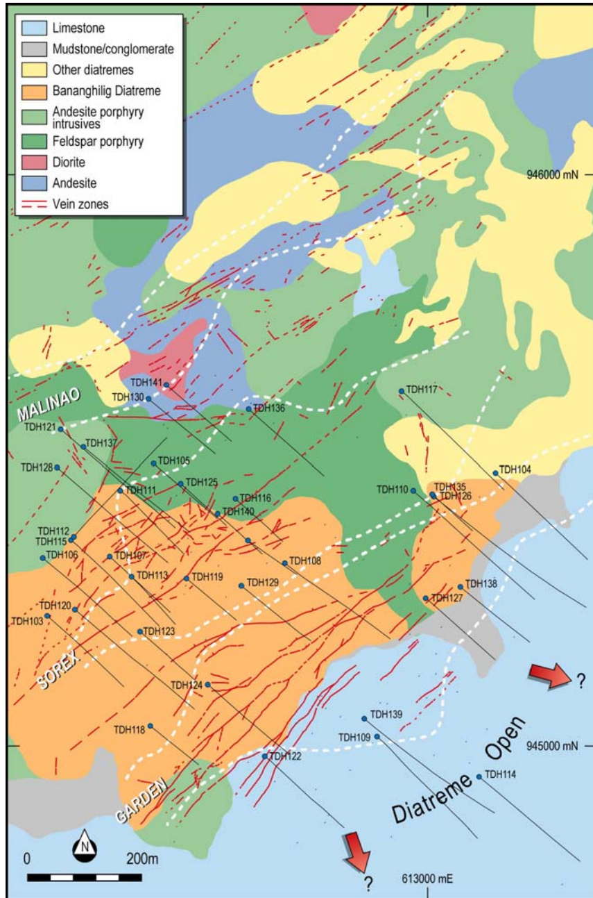
Figure 1. Geological interpretation map showing drill hole locations.
