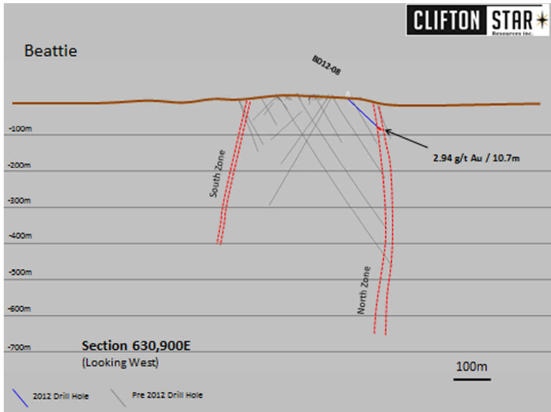
SECTION 630,900E
