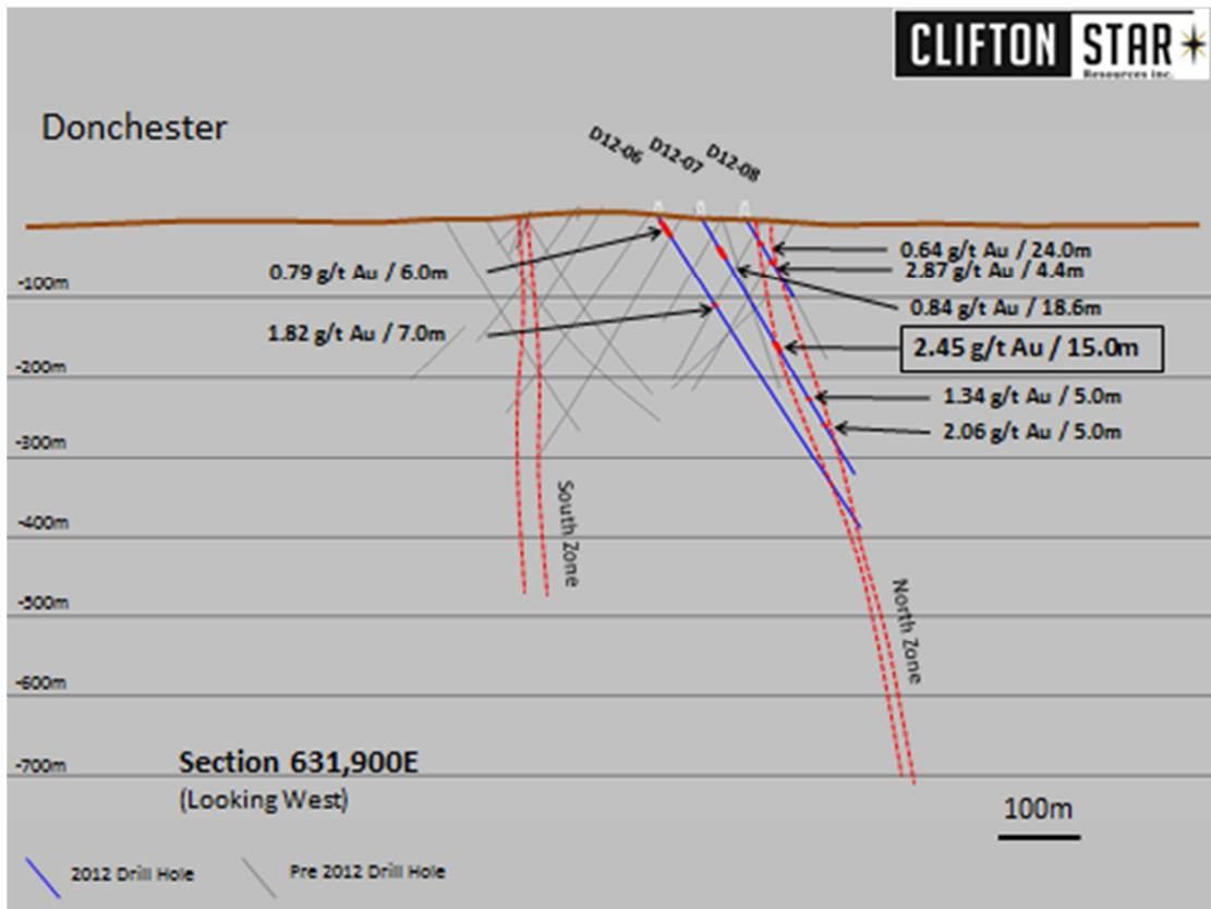
SECTION 631,900E
