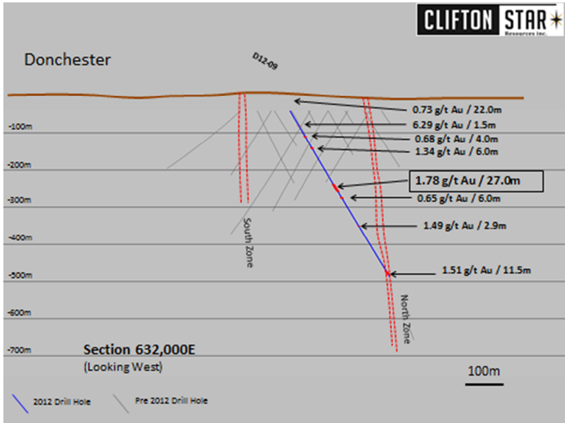
SECTION 632,000E
