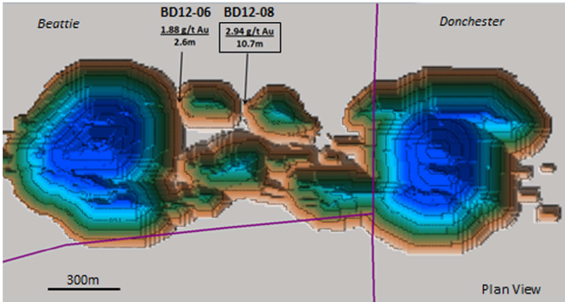
OPTIMIZED WHITTLE PIT, MAY 2012 – PLAN VIEW
