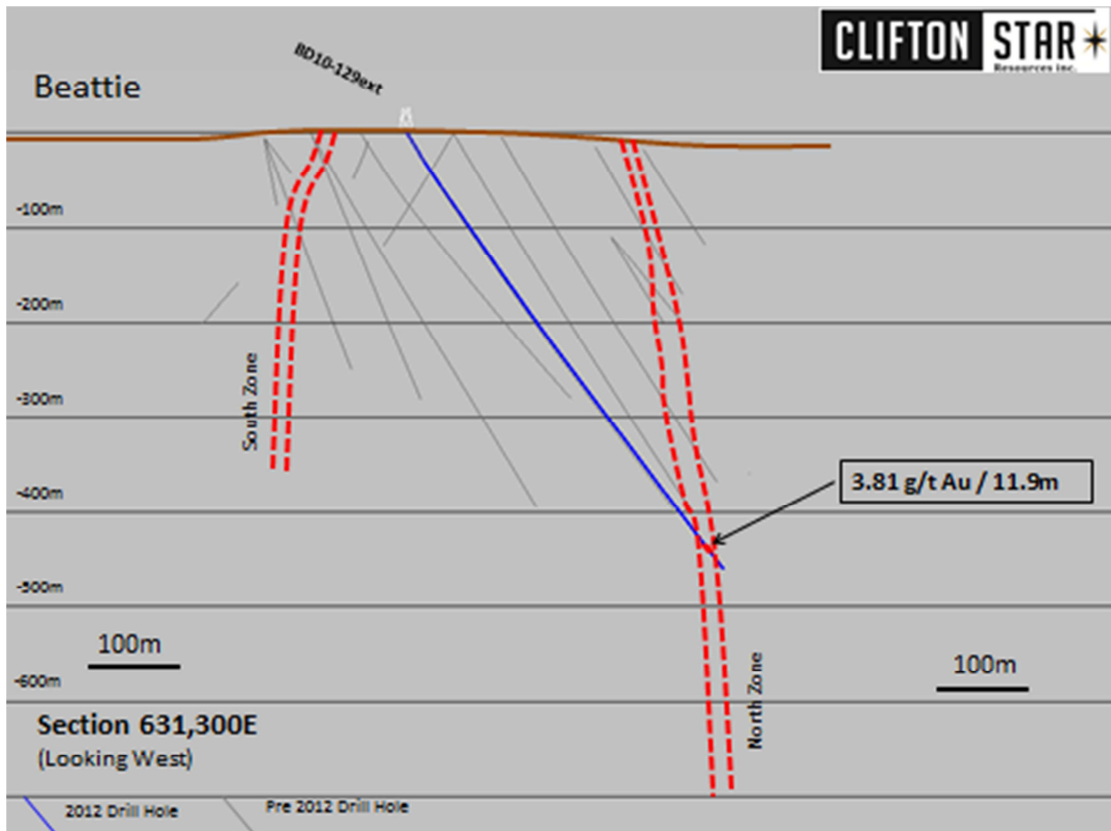
SECTION 631,300E
