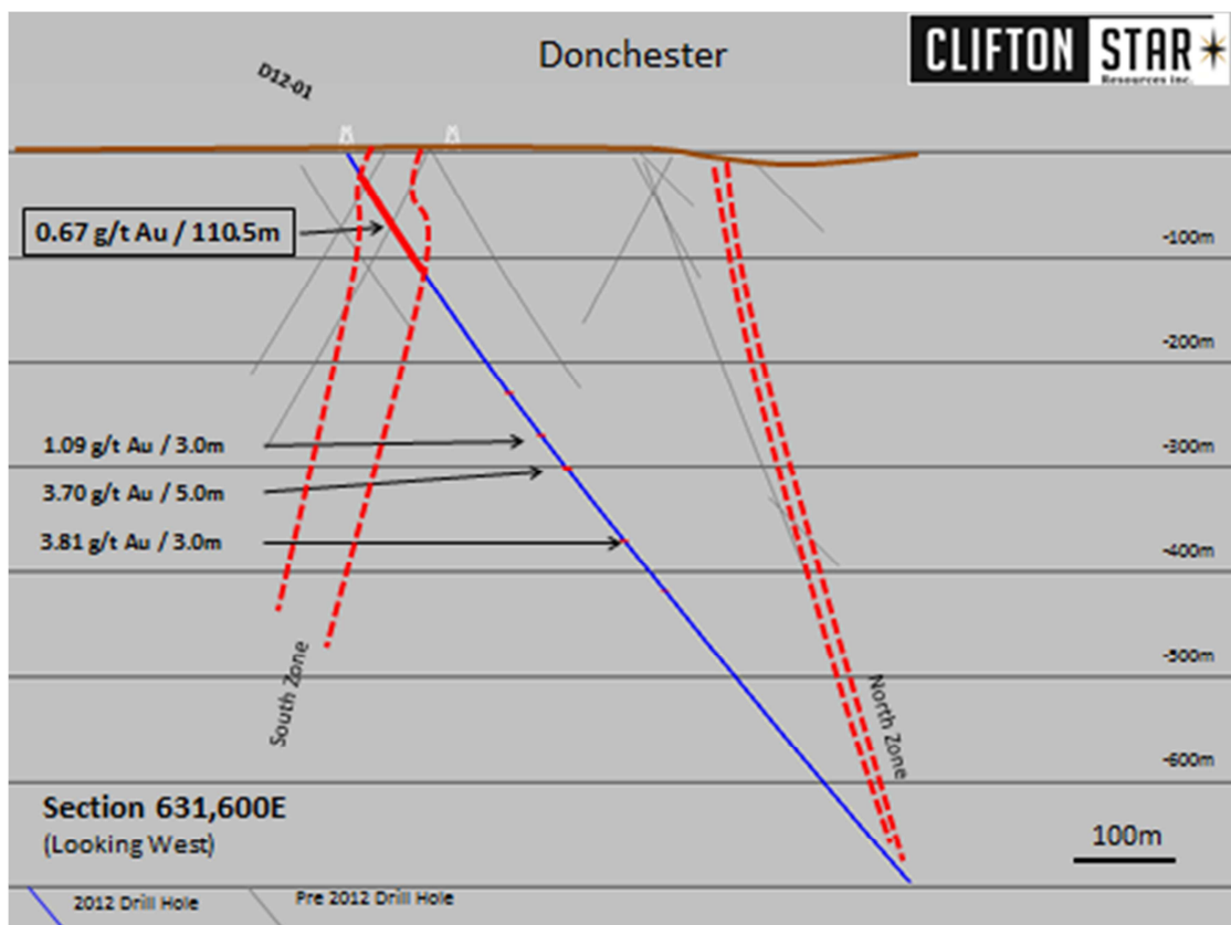
SECTION 631,600E
