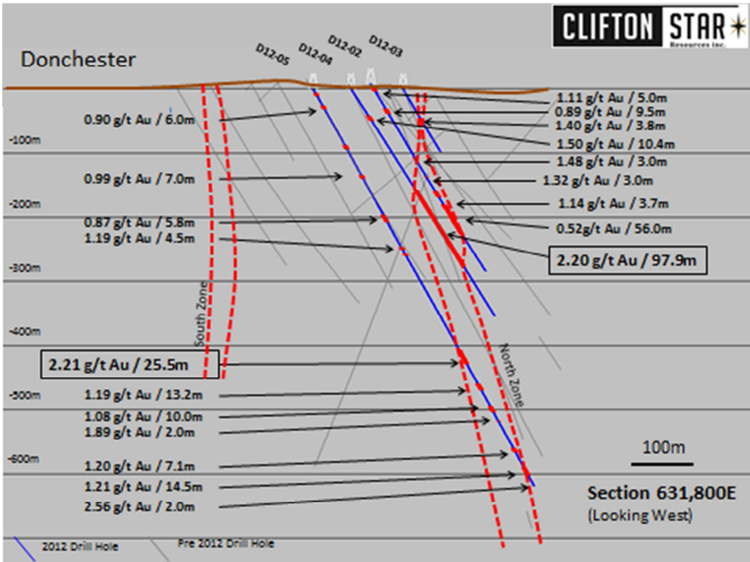
SECTION 631,800E
