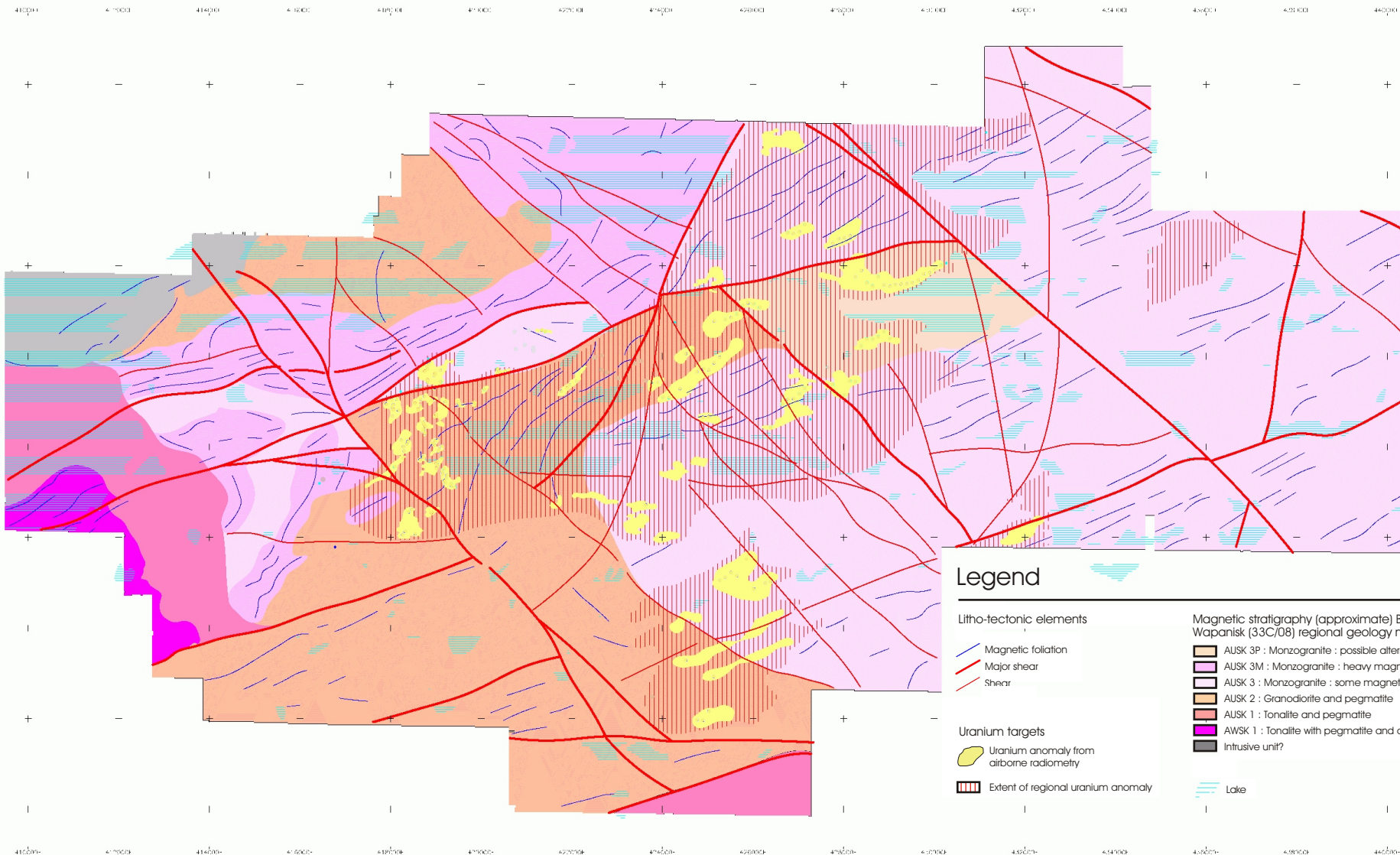
Uranium Bay Resources : Uskawanis Lake project : Aeromagnetic and radiometric survey Geophysical Interpretation Map
