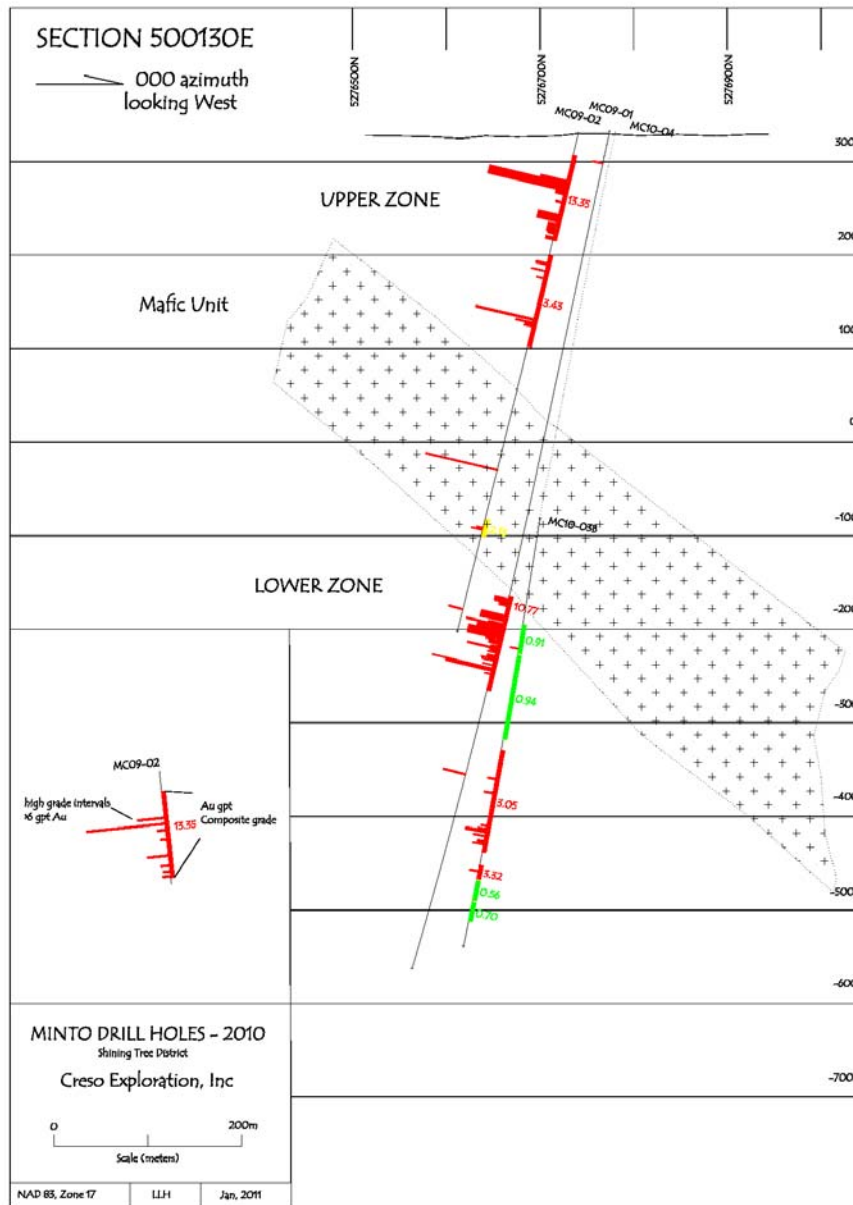
Figure 2 - Cross-section 500130E at the Minto Project.
