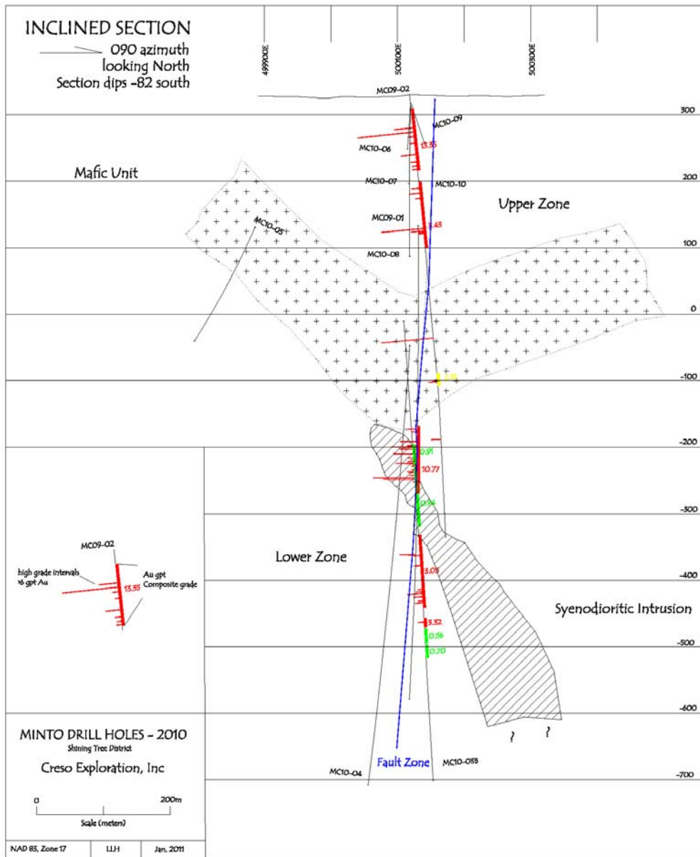
Figure 3 - Incline Section through the Minto Upper and Lower Zones.
