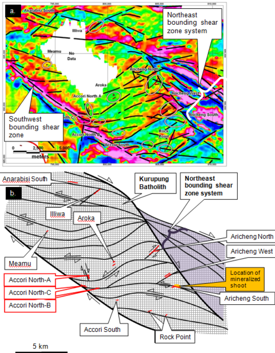
Figure 4 – Map of Magnetic Data and Interpreted Structures in Kurupung Batholith
