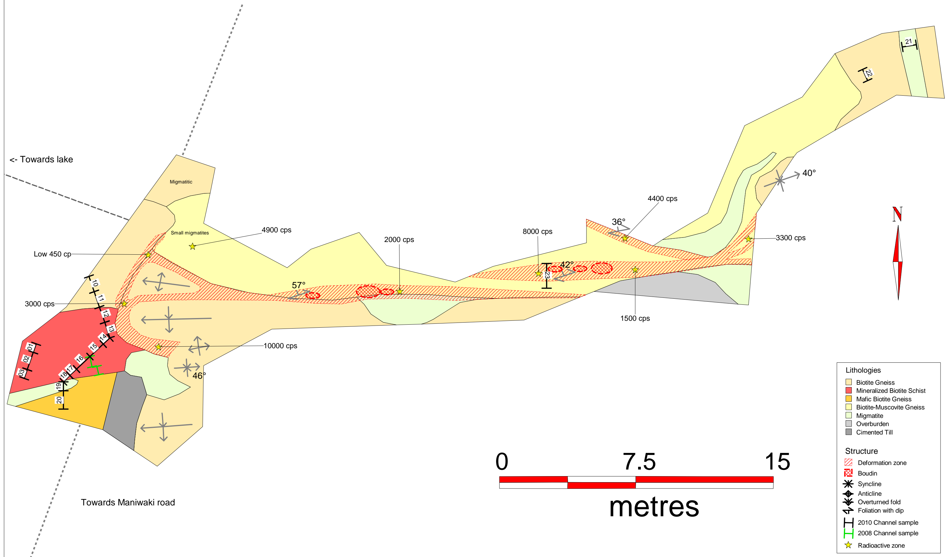
Figure 2. Geological map, 2010 trenching, Surprise showing
