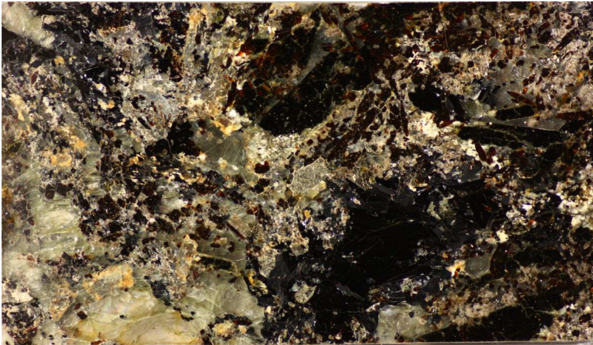
Fig. 2 T-780B 1 in natural light These slabs are rich in fergusonite and allanite (black). In addition, there is another Y, Nb, Ti oxide adjacent to fergusonite and rimming fergusonite. Its identification is still under investigation, but the EDS plots favor the mineral euxenite (Y) – (Y,Ca,Ce,U,Th) (Nb,Ta,Ti) 2 O 6 . Slab dimensions = 4.5 X 2.5 cm.
