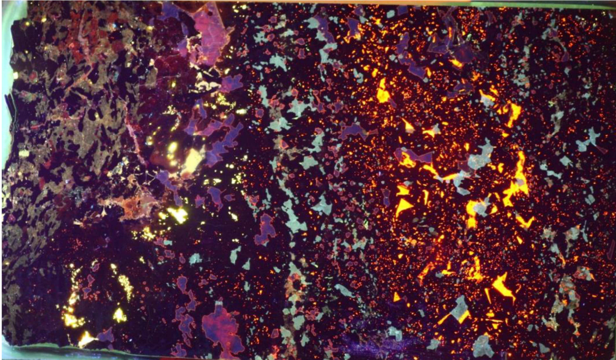
Fig. 3 T-780D in cathodoluminescence All of the light greenish-blue luminescing grains are xenotime. The orange grains are calcite, and the yellow grains are apatite. The rocks also contain allanite and cheralite (Ca-monazite). Slab dimensions = 4.5 X 2.5 cm.
