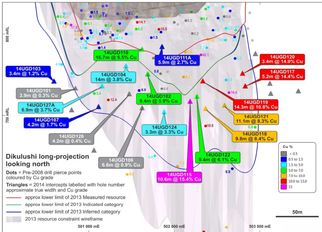
Figure 1: Dikulushi long projection (looking north) showing 2014 resource definition drill results (to end of September 2014)
