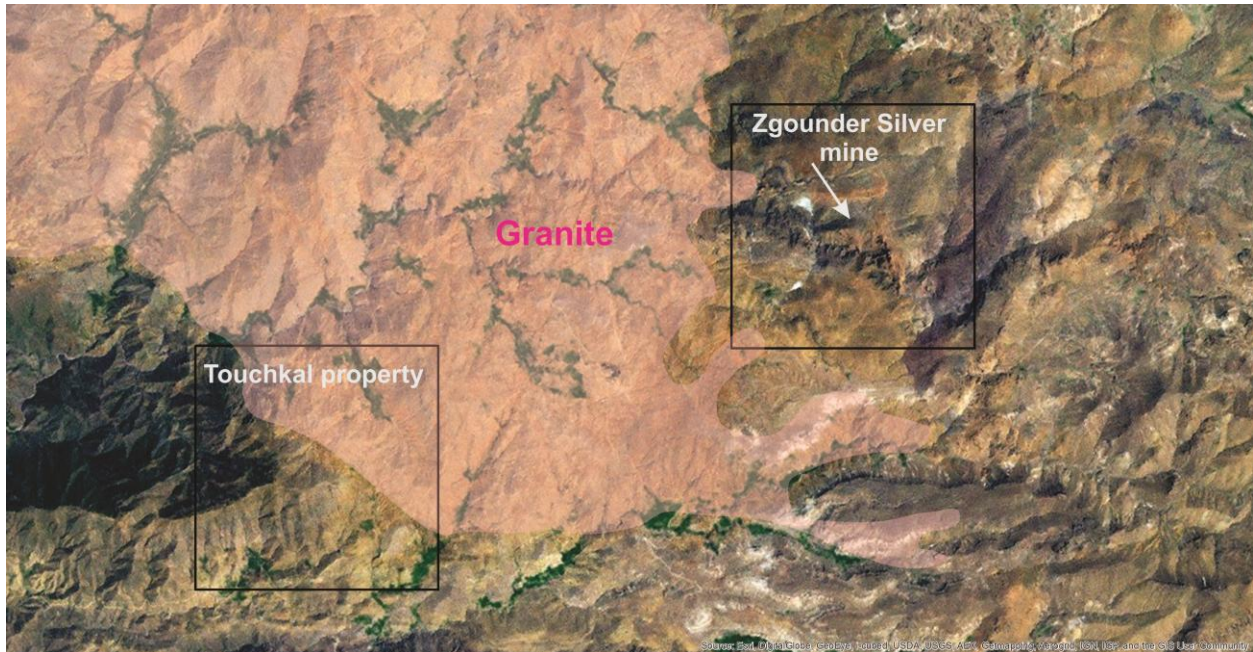
Satellite view of Zgounder area and location of Maya's properties in relation to the Askaoun granite pluton.
