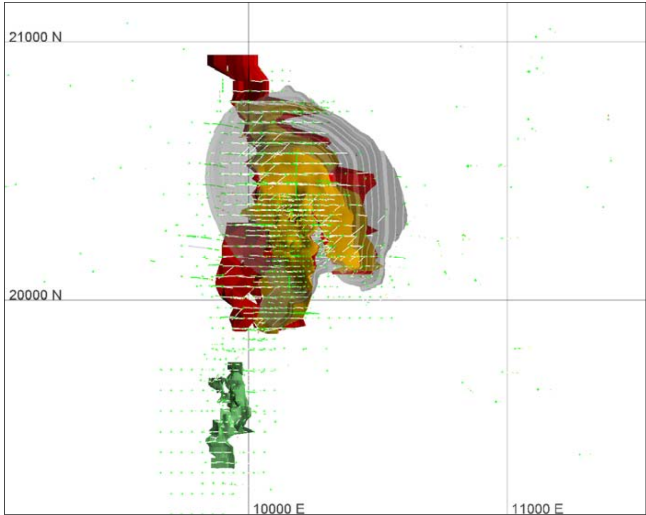
Figure 2. 2007 Main Flat Zone in gold, expanded Main Flat Zone shown in red, Sutuba extension to Sabodala shown in green, 2007 ultimate pit design in gray
