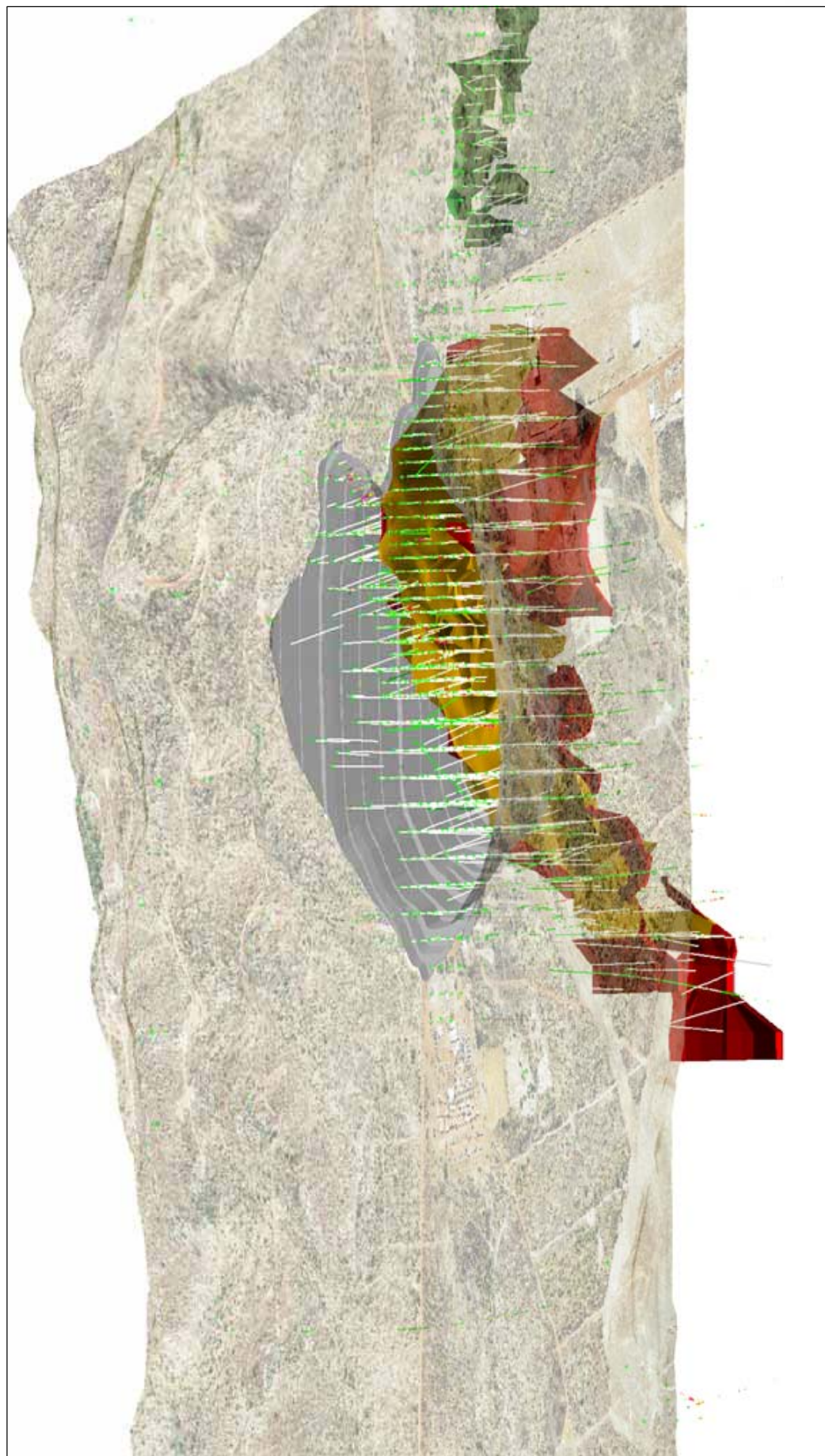
Figure 3. 2007 Main Flat Zone in gold, expanded Main Flat Zone shown in red, Sutuba extension to Sabodala shown in gray, 2007 ultimate pit design in gray
