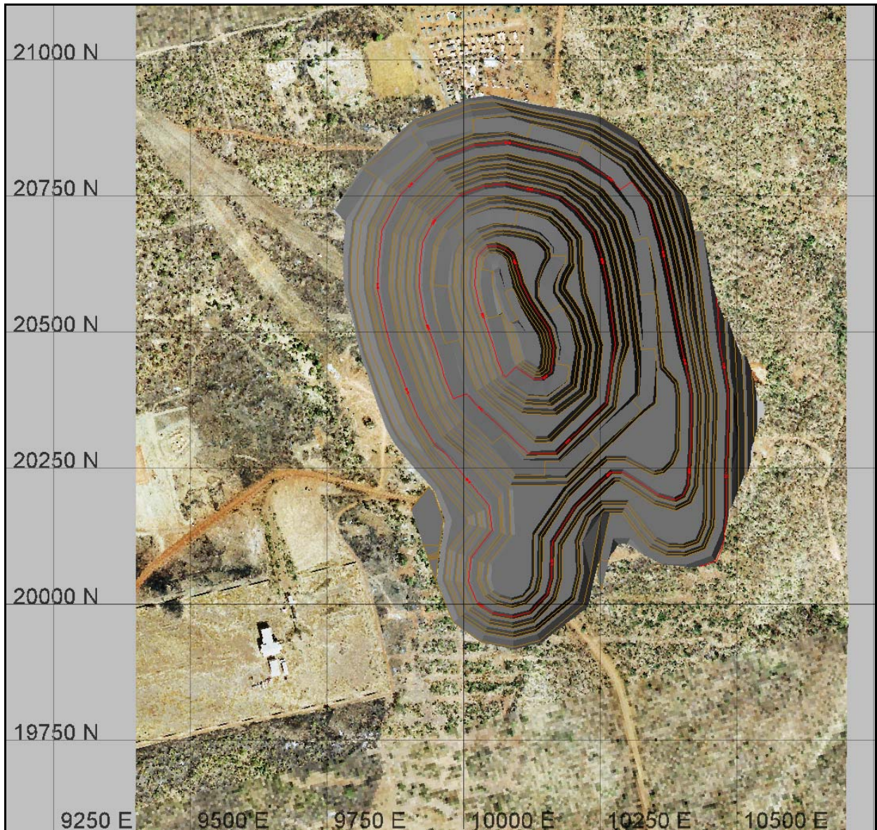
Sabodala 2008 new pit design
