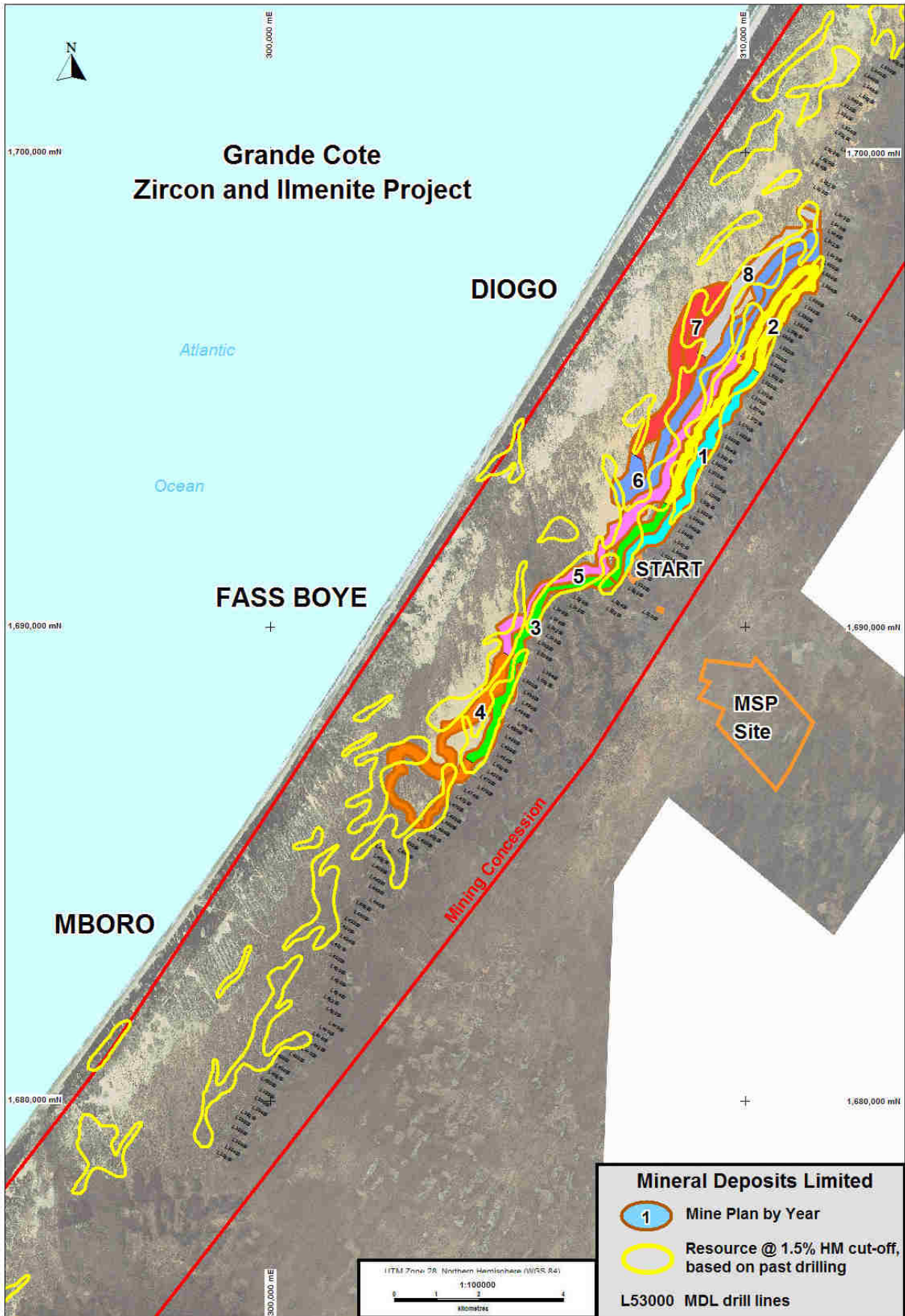
Diogo Mine Plan Showing Dredge Mining Path
