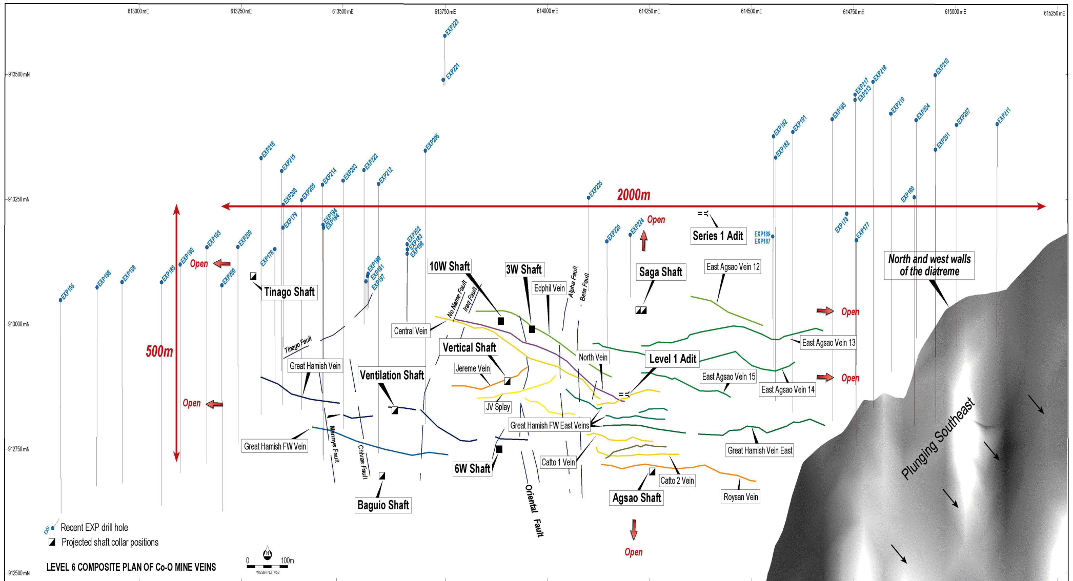
Figure 1. Map of the Co-O Mine Level 6 plan showing the locations of new drill holes EXP176 to EXP225
