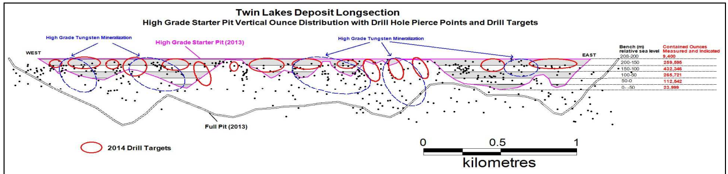
Figure 3: Twin Lakes Deposit Long Section – High Grade Starter Pit Vertical Ounce Distribution with DDH Pierce Points and Drill Targets
