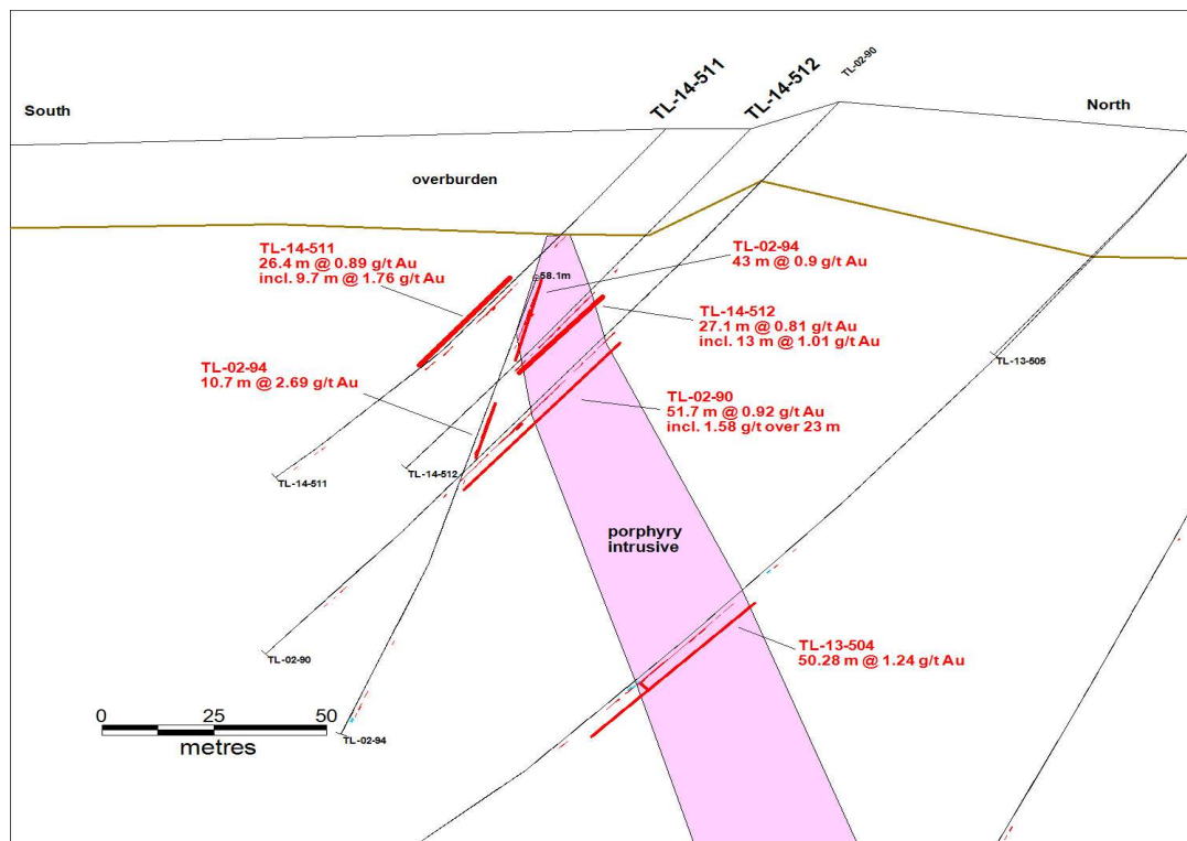
Figure 5: 2014 Drill Hole Cross Sections
