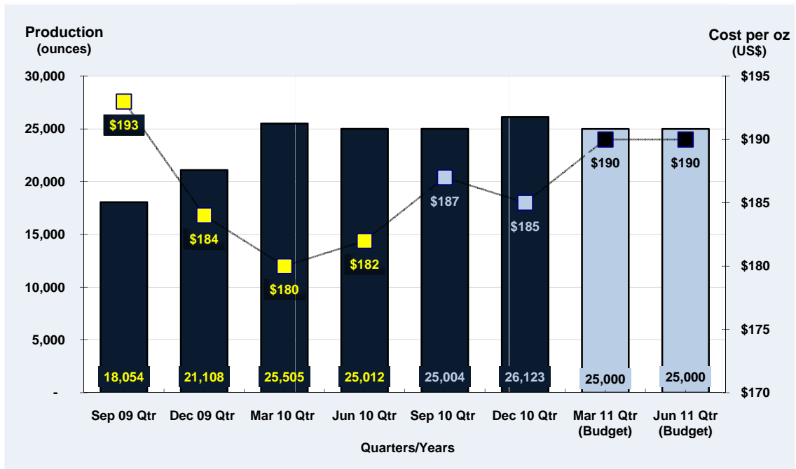
Graph 1. Co-O quarterly production graph with unit costs (Actual-fiscal year 2009/10, actual-Sep and Dec 2010 quarters and forecast-remainder fiscal year 2010/11).
