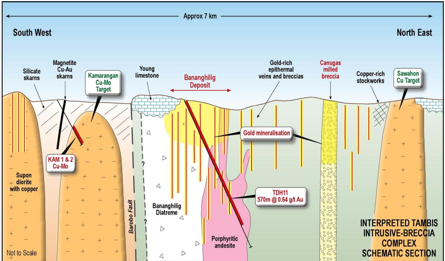
Figure 4. Interpreted Tambis intrusive-breccia complex schematic section
