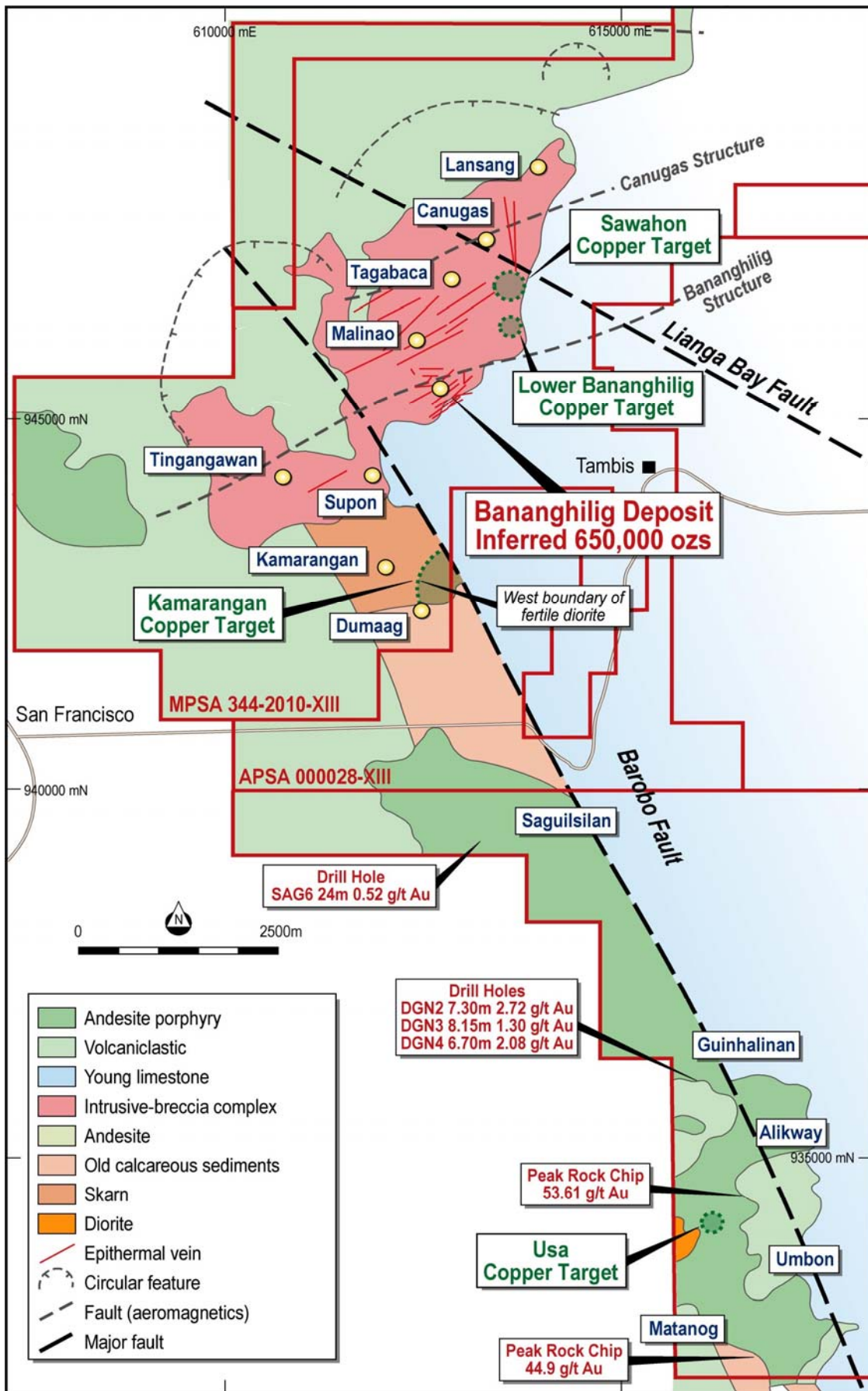
Figure 1. Regional geology map of the Tambis district and Barobo Corridor
