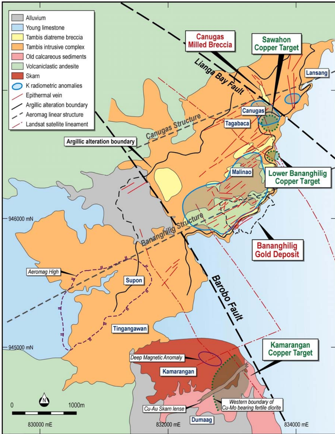
Figure 2. Map of the Tambis intrusive-breccia complex showing the generalised veins and copper targets
