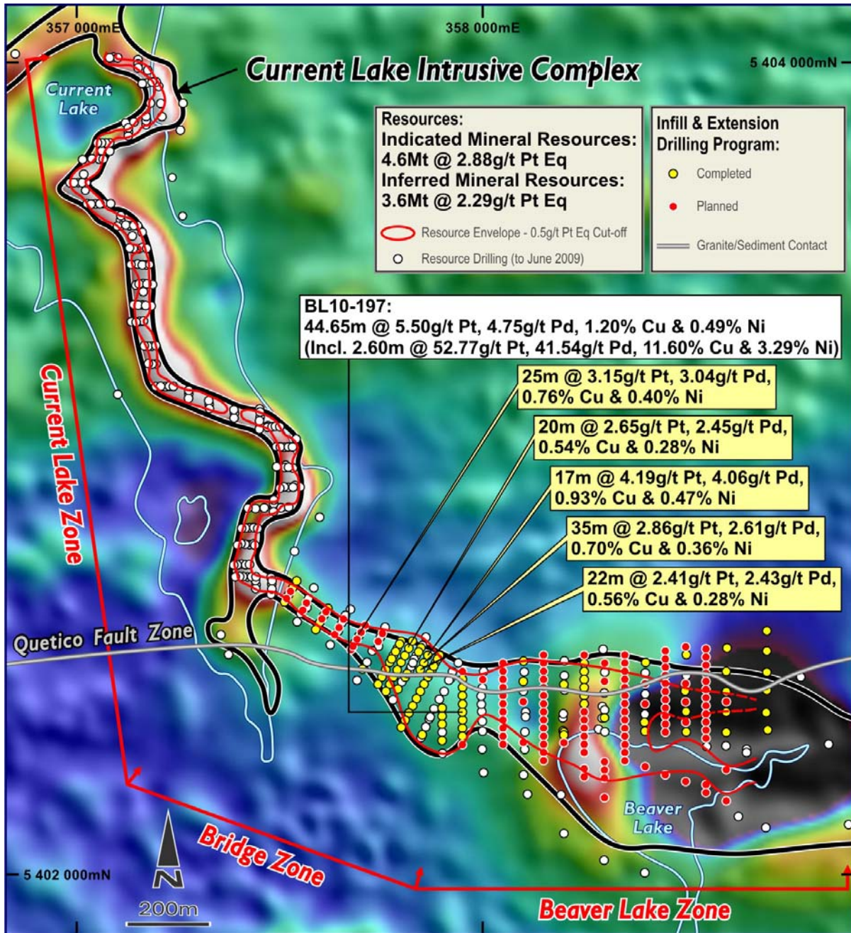
Current Lake Intrusive Complex, Magnetics and Drilling, showing drilling results for BL10-197 and other results recently reported in Magma's December 2009 quarterly report (available at www.magmametals.com.au ).
