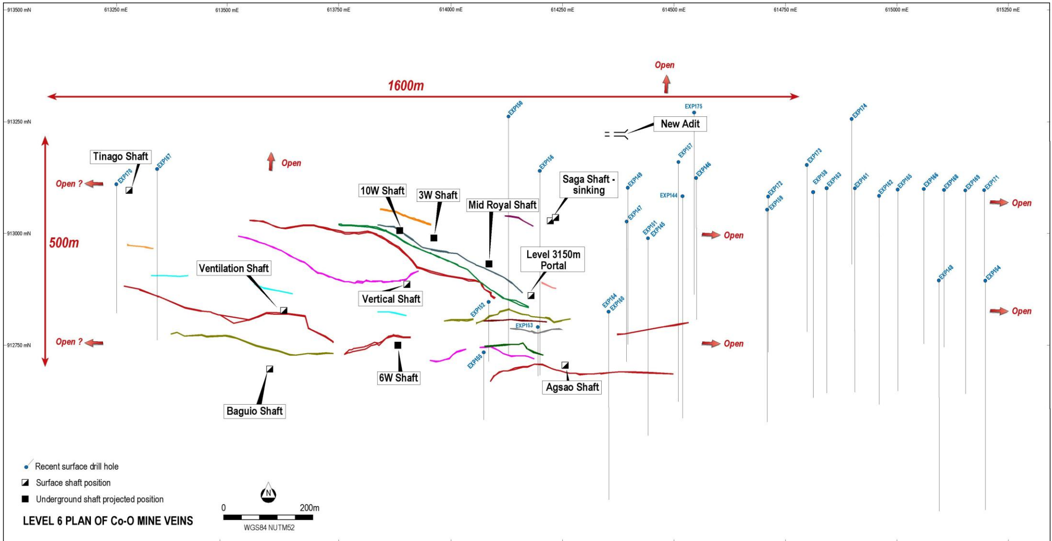
Figure1. Map of the Co-O Mine Level 6 plan showing the locations of new drill holes EXP146 to EXP175.
