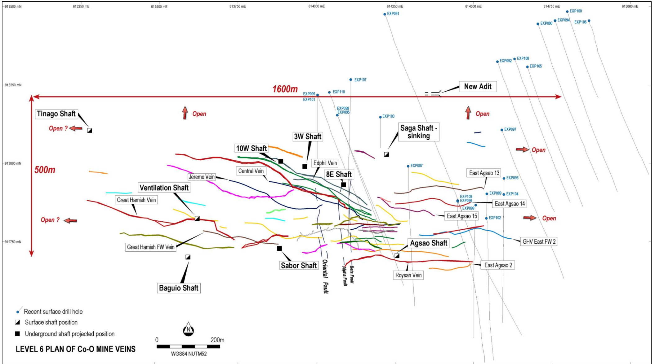
Figure 1. Map of the Co-O Mine Level 6 plan showing the locations of new drill holes MD306 to MD308, and EXP 065 to 086
