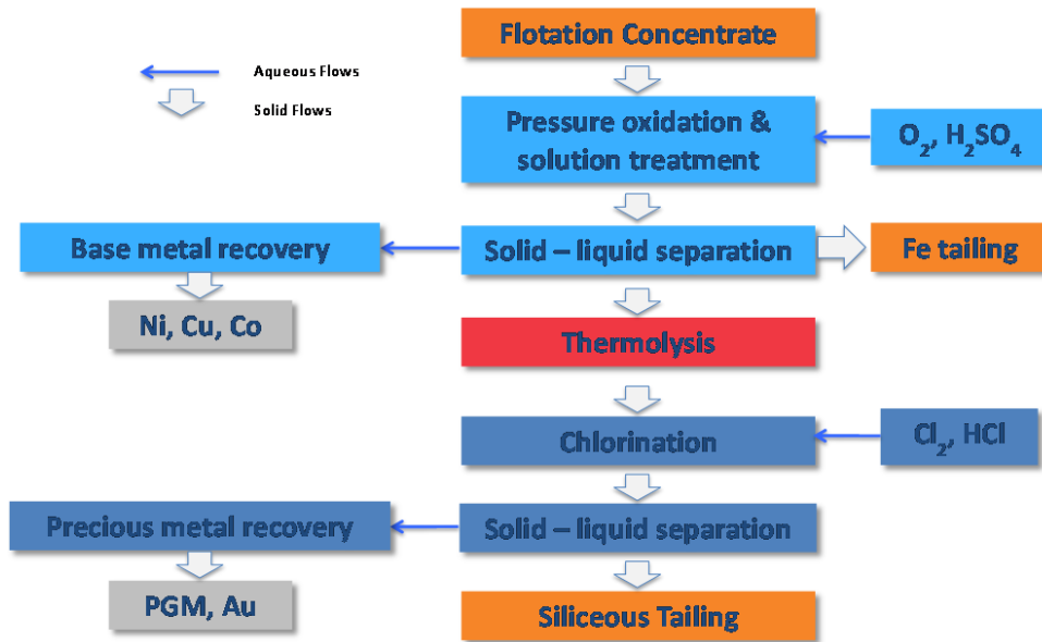
Figure 4 - Kell Process block flow diagram
