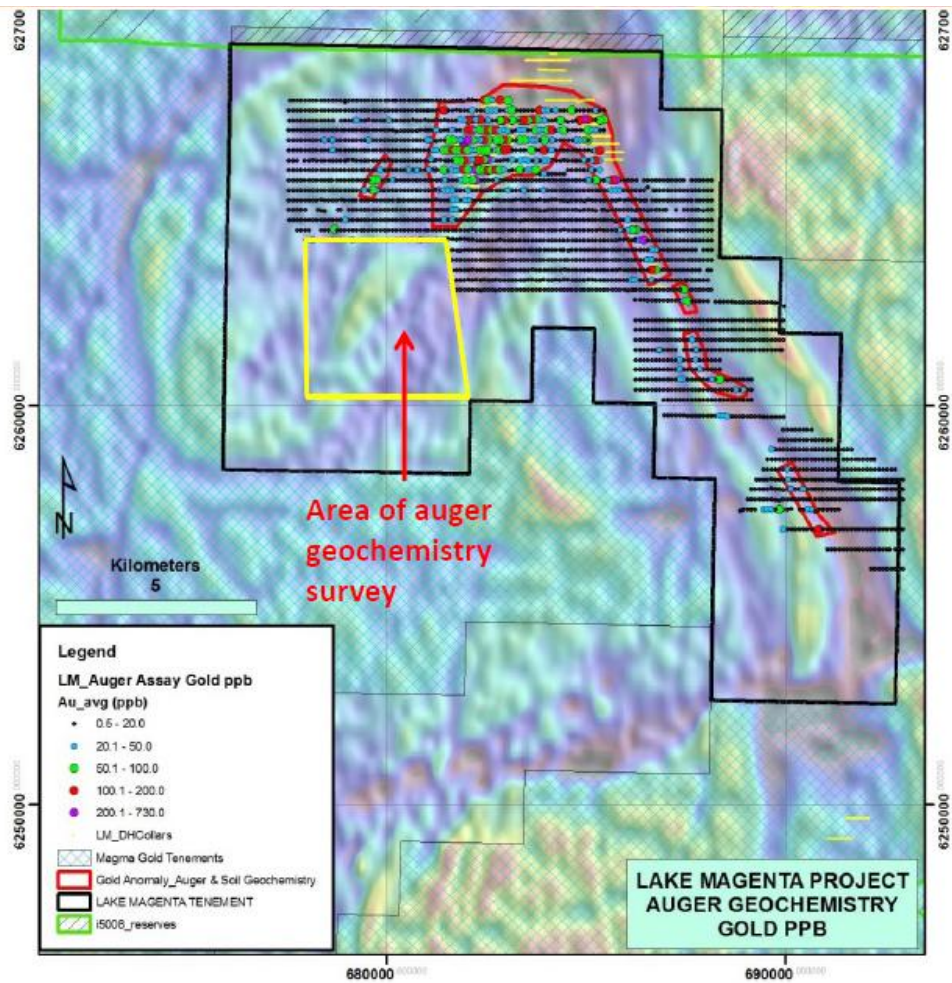
Figure 8. Lake Magenta gold anomalies and the planned auger geochemistry survey.
