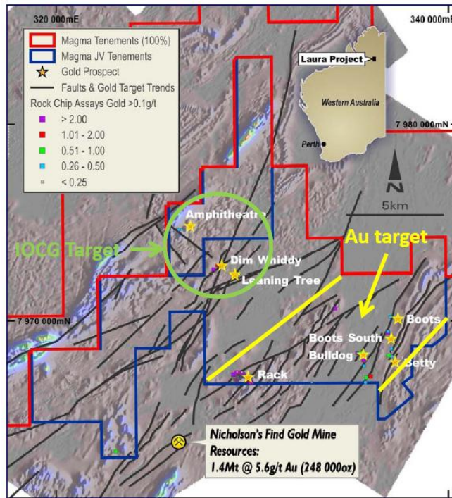
Figure 9. Laura River project showing the IOCG target to be covered by the planned auger geochemistry survey.
