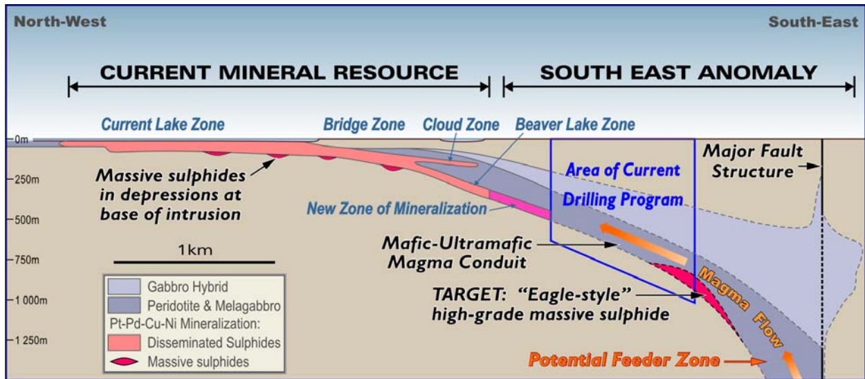
Figure 2. Conceptual long-section model of the Current Lake Intrusive Complex illustrating the area of current drilling and the potential massive sulphide exploration target
