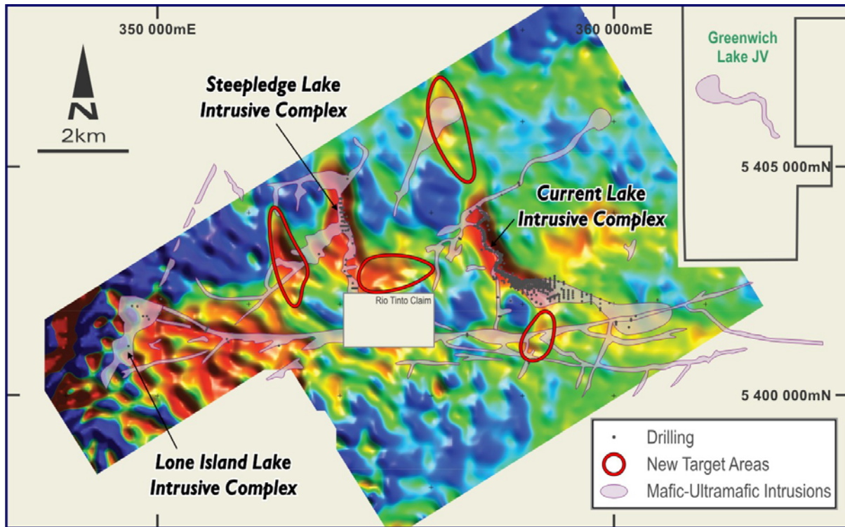
Figure 2. ZTEM survey of intrusive complexes in the TBN project showing new target areas.
