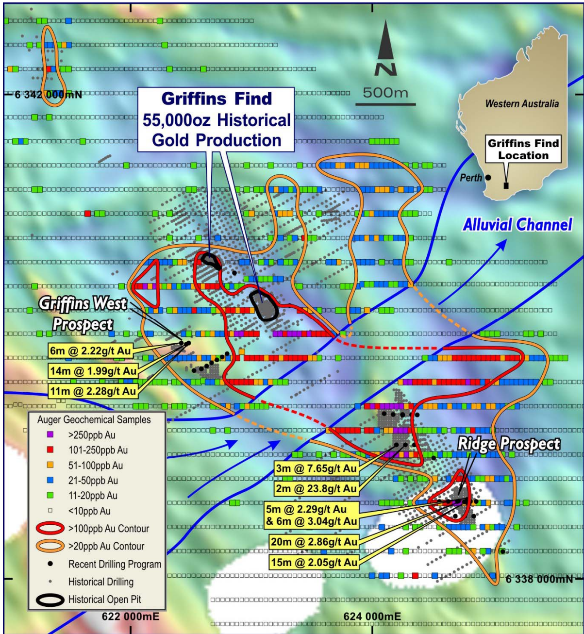
Figure 1. Magnetic image showing auger geochemical survey gold results and previously announced Magma drilling results at Griffins Find.
